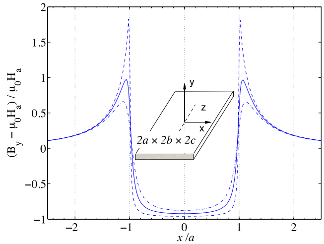
FIG. 3. The distribution of B_{\perp} across the width of the superconducting beam, at three different heights y above the surface, such as calculated for an aspect ratio b/a = 0.1 . Different lines correspond to y/a = 0.01 (dashed), 0.05 (continuous), and 0.1 (dotted-dashed). In all cases, a uniform applied magnetic field (0, H_a, 0) is assumed.
