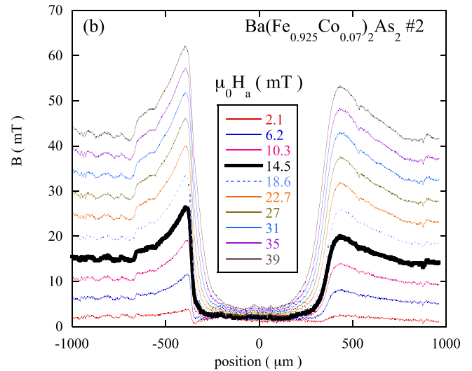
FIG. 1. (a) MOI of screening by \text{Ba}(\text{Fe}_{0.925}\text{Co}_{0.075})_2\text{As}_2 crystal #2, at \mu_0 H_a = 10\ \text{mT} , after zero-field cooling to 10 K. The rectangular outline of the crystal is clearly seen. The garnet has been purposely placed obliquely so that the sample-to-garnet distance is smaller along the top edge than along the bottom edge. (b) Profiles of the perpendicular flux density at successive applied fields, averaged over the strip between the two red lines in (a), after calibration of the luminous intensity. The heavy line indicates the first profile after flux penetration. The abscissa runs from the upper to the lower part of panel (a).
