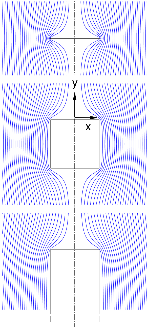
FIG. 2. Theoretical magnetic field lines surrounding ideal superconducting beams of rectangular cross section, in the Meissner state. Results are shown for aspect ratios b/a = 0.001, 1, and 10 and are obtained from Eqs. (2) and (3).
