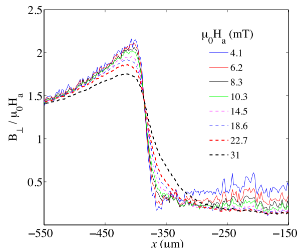
FIG. 6. Renormalized flux profiles over Ba(Fe 0.0925 Co 0.075 ) 2 As 2 crystal #2, for 4.14 < \mu_0 H_a < 30.95 mT, at T = 11 K.
