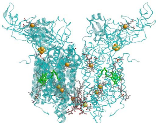
Figure 2: Structure of the Cyt b_6f dimer. PDB ID: 2E74 17 . Chlorophyll a molecules are highlighted in green. Iron atoms of hemes and iron-sulfur clusters are highlighted in gold. Cyan: protein. Orientation factor is 0.92 and the Mg-Mg distance is 6.1 nm.
