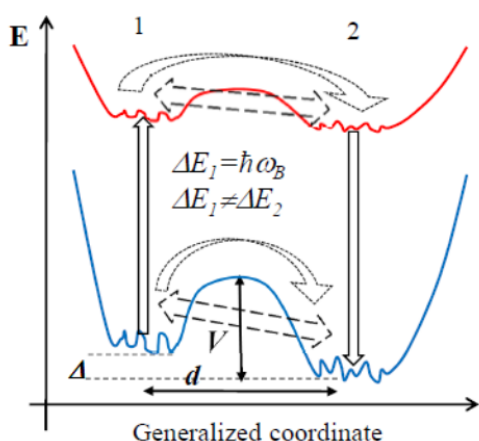
Figure 1: Energy landscapes of a pigment-protein system in ground (blue) and excited (red) electronic states. Two tiers of the protein energy landscape are shown. Vertical arrows indicate
