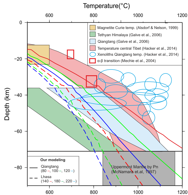
Figure 10. Temperature in depth from calculated models compared with known data [Mechie et al., 2004—red squares; Galve et al., 2006 blue and green areas; Hacker et al., 2014 purple area and blue empty ellipses]. Thin solid lines represent our modeling results for the temperature distribution in Qiangtang for the LAB: red 80-km, green-100 km, blue-120 km. The dashed lines indicate Lhasa temperatures (red-140 km, green-180 km, and blue-220 km).
