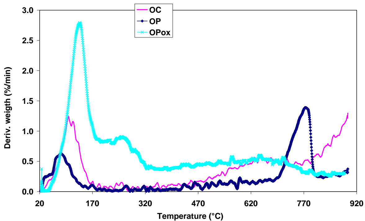
Figure S1. Thermogravimetric profiles of the nanoporous carbons studied obtained in inert atmosphere.
