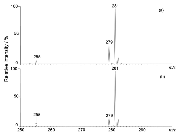
Figure 1. TI-EASI(-)-MS of (a) Cebo and (b) Bellota hams.
