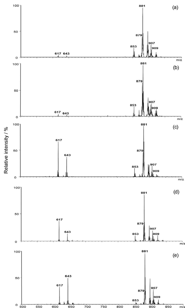
Figure 2. TI-EASI(+)-MS of (a) Parma; (b) Serrano; (c) Cebo; (d) Recebo and (e) Bellota hams.
