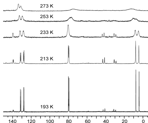
Figure 4. ^{31}\text{P}\{^1\text{H}\} NMR spectra of the reaction of 3 with one equiv. of \text{P}(\text{OMe})_3 in acetone- d_6 at various temperatures.
