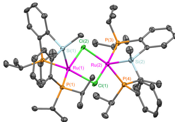
Figure 1. Crystal structure of complex 1 at 50% probability level. The hydrogen atoms are omitted for clarity. For bond distances and angles see Supporting Information.
