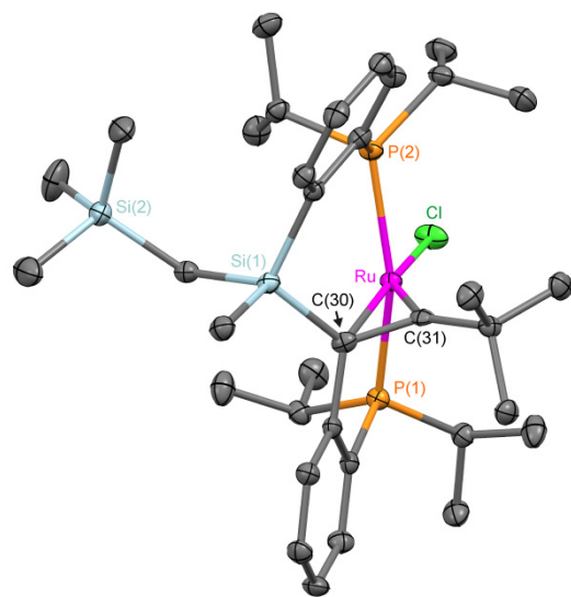
Figure 7. Crystal structure of complex 13 at 50% probability level. The hydrogen atoms are omitted for clarity. For bond distances and angles see Supporting Information.
