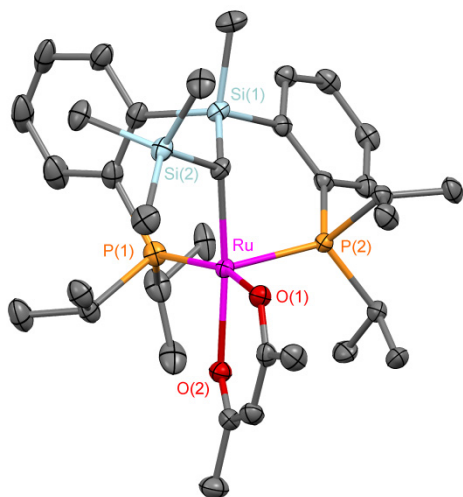
Figure 6. Crystal structure of complex 9 at 50% probability level. The hydrogen atoms are omitted for clarity. For bond distances and angles see Supporting Information.
