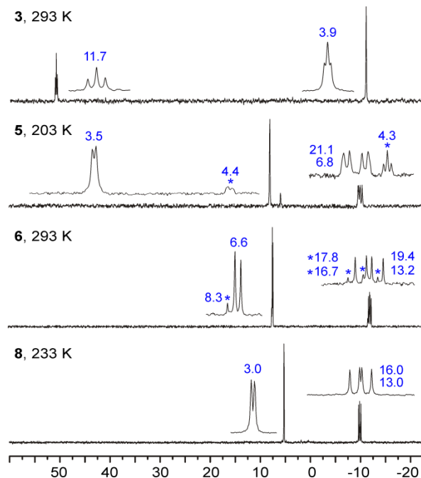
Figure 5. ^{29}\text{Si}\{^1\text{H}\} NMR spectra of 3 and the products of its reactions with \text{P}(\text{OMe})_3 ( 5 ), CO excess ( 6 ) and \text{NCMe} excess ( 8 ). In blue J_{\text{SiP}} coupling constants. Asterisks denote signals and constants corresponding to the minor products.
