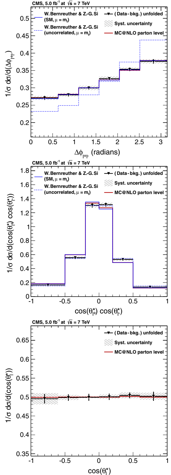
FIG. 1 (color online). Background-subtracted and unfolded differential cross sections for \Delta\phi_{\ell^+\ell^-} , \cos(\theta_{\ell^+}^*)\cos(\theta_{\ell^-}^*) , and \cos(\theta_{\ell^*}^*) . The error bars represent statistical uncertainties only, while the systematic uncertainty band is represented by the hatched area. The bin contents are correlated due to the unfolding.
