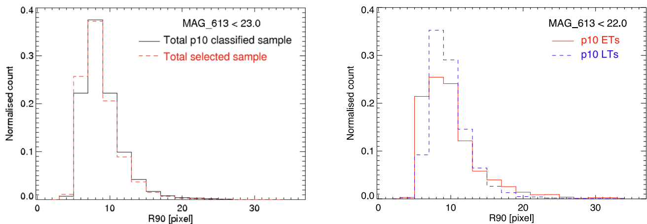
Figure 10. Normalized distributions of radius at 90 per cent of flux for: total selected (red dashed lines) and p_{10} classified (black solid lines) samples (left-hand panel), and ET (red solid lines) and LT (blue dashed lines) galaxies (right-hand panel).
