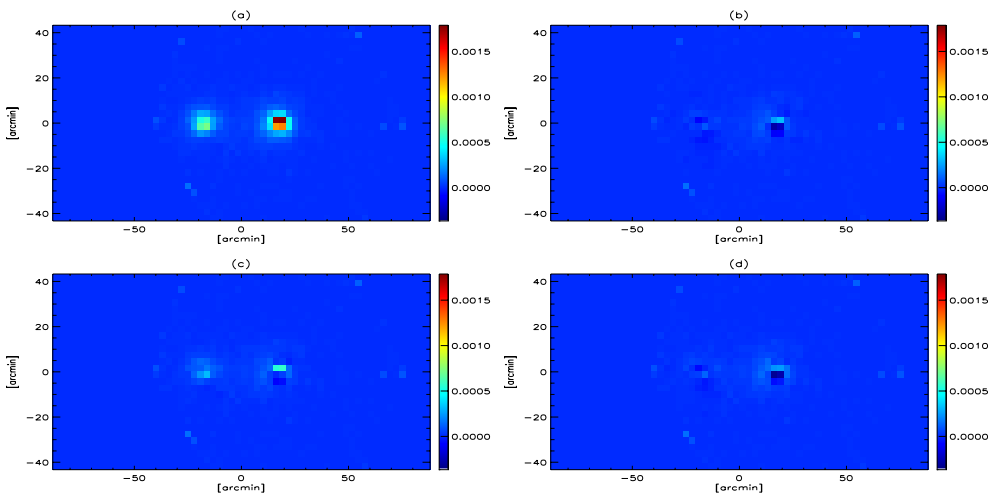
Fig. 5. X-ray data and residuals of the best-fit cluster model for the A399 and A401 pair of clusters. a) ROSAT map; b) residuals for the GNFW2 model; c) residuals for the GNFW1 model; and d) residuals for the \beta model.
