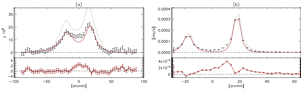
Fig. 6. 1D a) tSZ and b) X-ray profiles and residuals for the best-fit models of the A399 and A401 clusters. The red curve corresponds to the GNFW2 model. The dotted lines are the model from Sakelliou & Ponman (2004).
