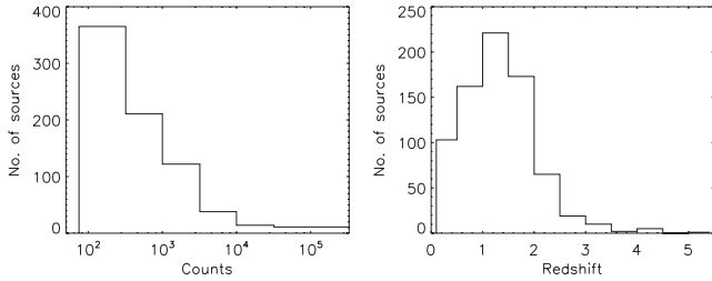
Figure 1. Histograms showing the net counts and redshift distributions of the sample used here, and described further in S11.
