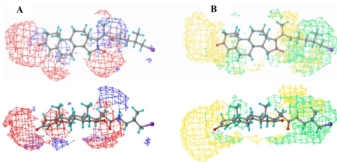
Figure 3. Electrostatic and steric contours mapped onto compound 15 .
