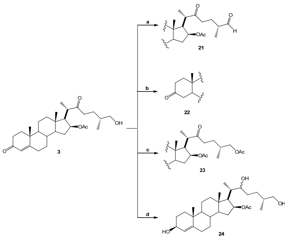
Scheme 3. SN-1 derivatives 21–24 produced by modifications made to the side chain and A-ring. SN-1 ( 3 ).
