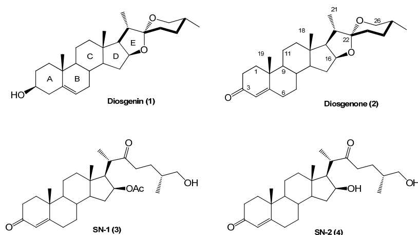
Figure 1. Structure of diosgenin and diosgenone, SN-1 and SN-2 S. nudum sapogenin.
