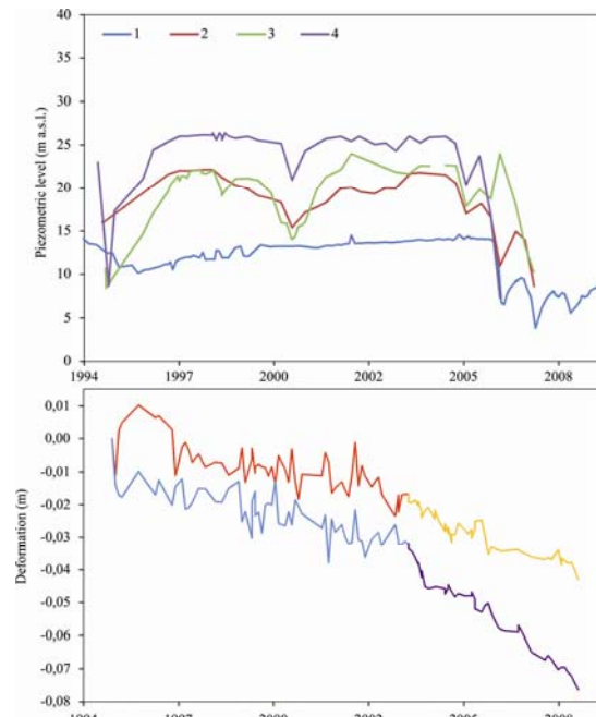
Figure 5. (Upper) piezometric level in several piezometers of the Vega Baja of the Segura River, (Lower) Temporal evolution of two PSs. Piezometer are located in Figure 4. The selected PSs are located in the Orihuela city center (modified from [3]).
