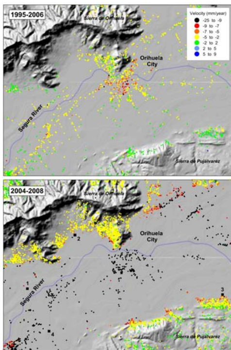
Figure 4. Deformation rates (in mm/year) along LOS for the periods 1995–2006 (Upper) and 2004-2008 (Lower) in the lower part of Segura River basin. Notice the high subsidence affecting the south area of the Orihuela City [3].
