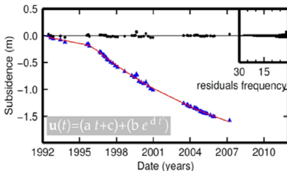
Figure 8. Ground surface deformation time series modeling (ground deformation, y-axis, versus date, x-axis) for the maximum detected subsiding point in the Alto Guadalentín basin. Linear plus an exponential decay model. Blue triangles are data points, red lines are model predictions and black dots are the residuals between data and model. In the upper-right corner of each subplot is a small rectangle containing a residual [1].
