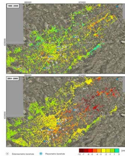
Figure 2. Total deformation estimated with SPN technique between July 1995 and December 2005. Bottom: Total deformation estimated with SPN technique between January 2004 and December 2008. Labels have been placed in those piezometers which were analyzed [2].
