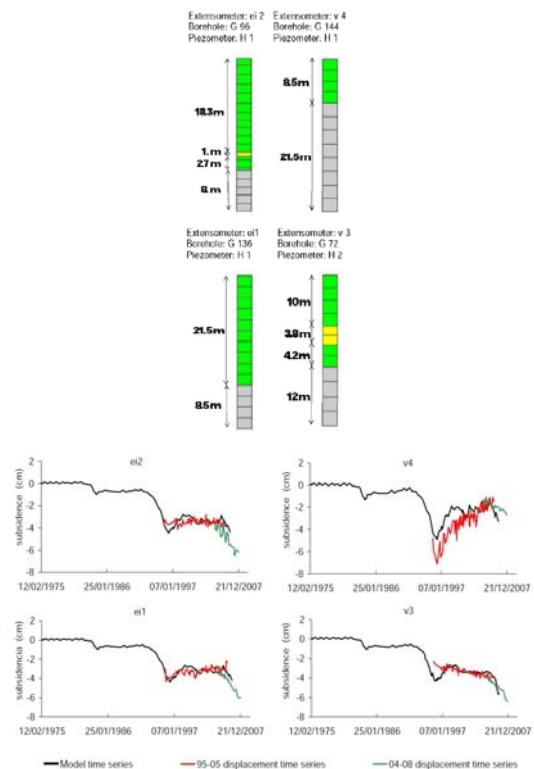
Figure 3. (Top) Finite element mesh of the considered soil columns. Green: clay; yellow: sand; gray: gravel. (Bottom) LOS projected time series of the deformation simulated with the model and observed with SPN (modified from [2]).
