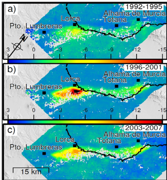
Figure 7. StaMPS/SBAS results in cm/yr. Surface LOS ground velocity for a) the period 1992-1995, b) period 1996-2001, and c) period 2003-2007. Note that the ground deformation follows the deflection of the river valley, a structural direction (EW to ENE-WSW) similar to a geophysical inferred local grabens and horsts [1].
