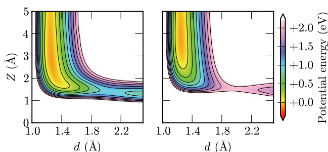
Fig. 8. Equivalent two-dimensional cuts of the CRP (left) and NN (right) PES representations similar to the upper panel of Fig. 5. The (d – Z ) elbow plots are shown for X_{\min} , Y_{\min} , \vartheta_{\min} and \varphi_{\min} - 90^\circ , i.e. the coordinates of the “bumps” identified in Fig. 7 backfolded in the irreducible wedge (see text).
