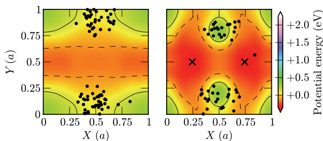
Fig. 7. Equivalent two-dimensional cuts of the CRP (left) and NN (right) PES representations similar to the lower panel of Fig. 5. The (X – Y ) plots correspond to Z_{\min} , d_{\min} , \vartheta_{\min} and \varphi_{\min} , i.e. they are cuts along the lateral plane through the NN global minimum at (X_{\min} = 0.25 a, Y_{\min} = 0.5 a, Z_{\min} = 2.14 \text{ \AA}, d_{\min} = 1.28 \text{ \AA}, \vartheta_{\min} = 90^\circ, \varphi_{\min} = 90^\circ) in the irreducible wedge ( cf. Fig. 2). Note that due to the symmetry of the angular coordinates ( \vartheta_{\min} , \varphi_{\min} ), a horizontal and vertical mirror plane perpendicular to the surface through the hollow site ( i.e. the center of the panels) is preserved from the clean Ag(100) surface symmetry within these cuts. Consequently, there is also a symmetry equivalent counterpart of the NN global minimum at (\bar{X}_{\min} = a - X_{\min}, Y_{\min}, Z_{\min}, d_{\min}, \vartheta_{\min}, \varphi_{\min}) . Both minima are marked by black crosses. The black circles correspond to trajectory data and show the respective positions of the molecular center in this cut plane (folded back into the unit cell) for molecules that pass closely through this cut plane, i.e. (Z, d, \vartheta, \varphi) \in [Z_{\min}, d_{\min} \pm 0.05 \text{ \AA}, \vartheta_{\min} \pm 30^\circ, \varphi_{\min} \pm 20^\circ] . Other than in the inset of Fig. 4), only equivalent trajectories starting from the same initial conditions with an incidence energy of 2.0 eV are included that dissociate on the CRP (left) but are reflected on the NN PESs (right).
