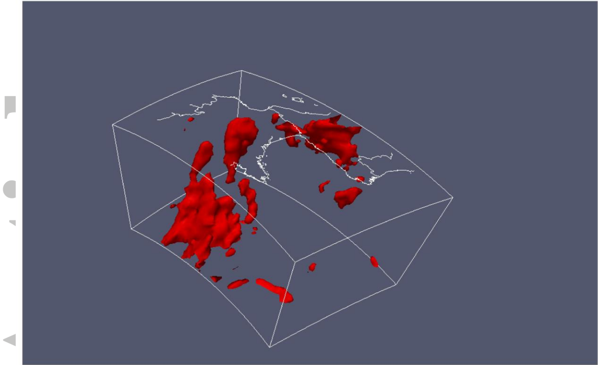
Figure 13. 3-D view of the isocontour corresponding to a perturbation of -0.75 % of the P velocity. The bottom of the box is at 900 km depth. The broad low velocity anomaly in the transition zone is not connected from the shallow asthenospheric anomaly beneath the Massif Central.
