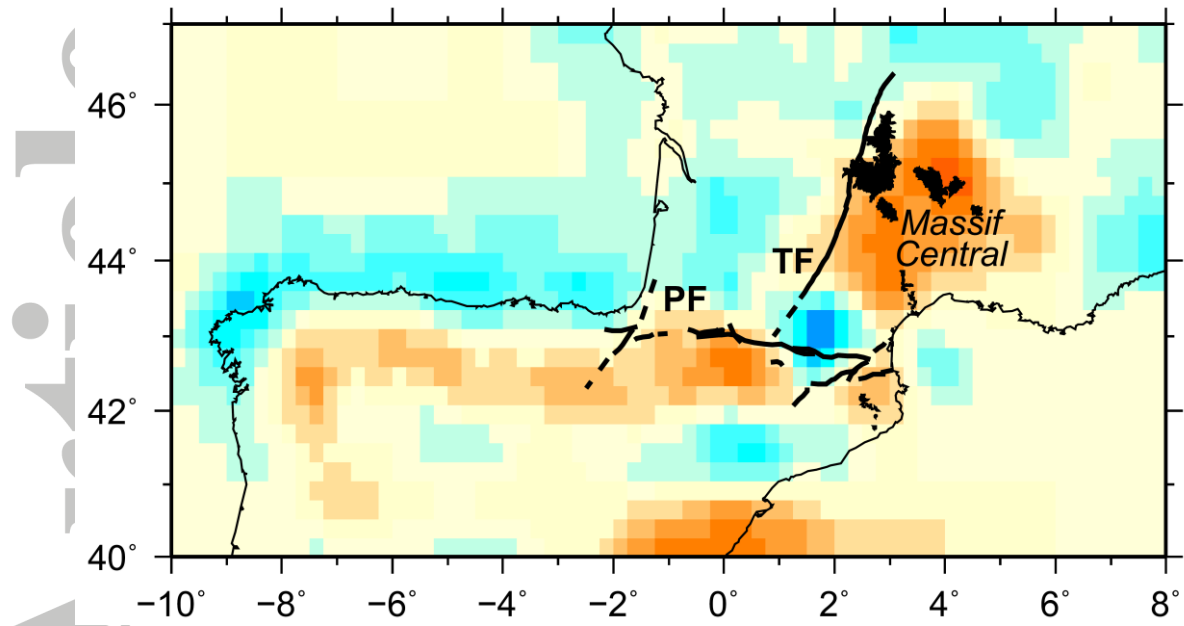
Figure 15. Map of P velocity anomalies between 125 and 150 km depth. The volcanic regions are the black shaded domains. The main faults in the Pyrenees are drawn with thin black solid lines while the Pamplona (PF) and Toulouse (TF) faults are drawn with thick black dashed lines.
