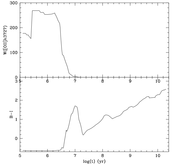
Fig. 8.— The evolution of the [OII] \lambda 3727 equivalent width and the B-I color with time after a single, instantaneous burst of star formation (the model has been kindly provided by G. Magris).
