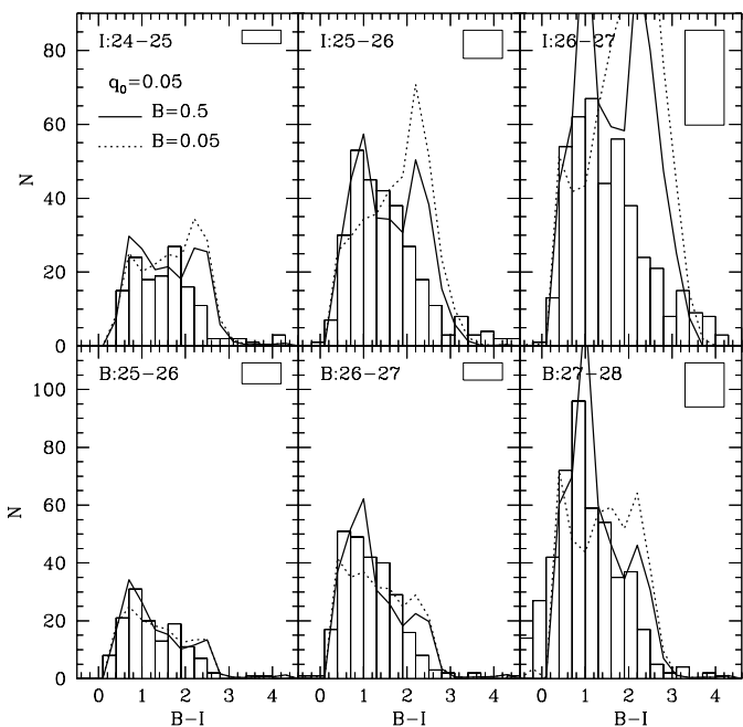
Fig. 3.— The same than Figure 3, but models now incorporate a population of dwarf galaxies with the star formation lasting 0.05 and 0.5 Gyr ( q_0 = 0.05 ).
