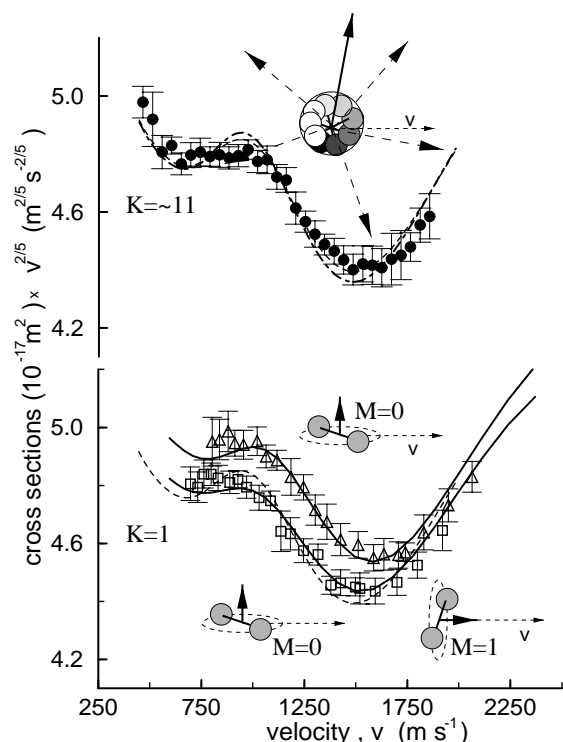
FIG. 1. Cross sections Q(v) for the O_2 - O_2 system (multiplied by v^{2/5} to emphasize the glory structure; see text) as a function of the beam velocity v . Upper panel: Scattering of a rotationally “hot” effusive beam of O_2 with a rotational distribution peaked around K \approx 11 . In this case, anisotropy effects due to the relative mutual orientations can be neglected: dot-dashed curve is calculated excluding spin-spin interactions, dashed curve is obtained considering the scattering on the three potential energy curves of singlet, triplet, and quintet character. Lower panel: Typical data for scattering of rotationally “cold” supersonic seeded beams of molecular oxygen at alignment ratios W_0/W_1 = 1/2 (squares) and 4 (triangles). Continuous curves are quantum mechanical close coupling calculations (see text). Dashed curve is as above and is repeated for comparison.
