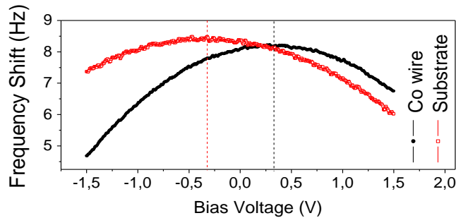
Figure 3.3: \Delta\omega vs bias. Frequency shift dependence on the tip-sample bias, obtained (black curve) in the central part of the stripe shown in the upper part of figure 3.2.a and (red curve) with the tip placed over the substrate.
