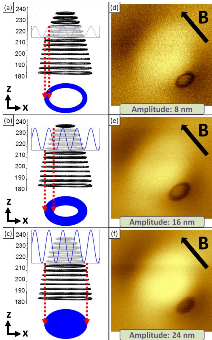
Figure 5.10: Dependence of the ring on the oscillation amplitude. (a)–(c) X-Z cross sections from figure 5.8.b ( z > 180 \text{ nm} is shown). (d)–(f) MFM images showing this effect, at a mean separation of 230 nm.
