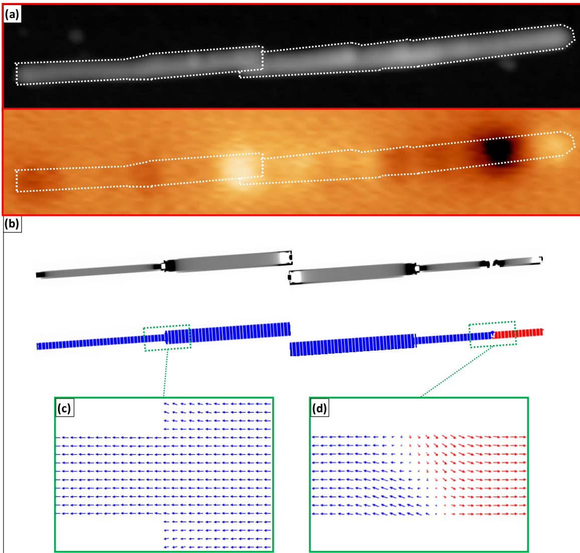
Figure 2.25: The demagnetized domain structure (II). (a) Nanowire highlighted in red in figure 2.23. The lateral size is 3 \mu\text{m} . (b) Two separately simulated nanowires reproducing the experimental data. The one on the left is in its equilibrium single domain state (see the monotonous blue contrast in the lower row), whereas the one on the right shows a dynamic snapshot with a domain wall. (c) & (d) Magnified images of the regions highlighted in (b).
