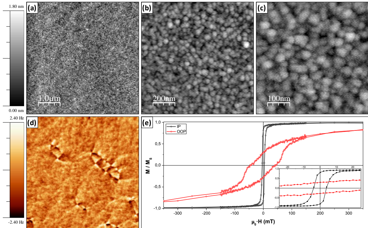
Figure 4.3: The cobalt coating. (a) (5 \times 5) \mu\text{m}^2 , (b) (750 \times 750) \text{ nm}^2 and (c) (375 \times 375) \text{ nm}^2 topographic images of a 20 nm thick Co layer grown onto an AFM chip (Nanosensors PPP) under the conditions used for coating the tip. (d) (5 \times 5) \mu\text{m}^2 MFM image of the same sample, showing a predominant IP magnetization with the presence of cross-tie domain walls. (e) In-plane (IP) and out-of-plane (OOP) hysteresis loops show the preference of the magnetization to remain IP.
