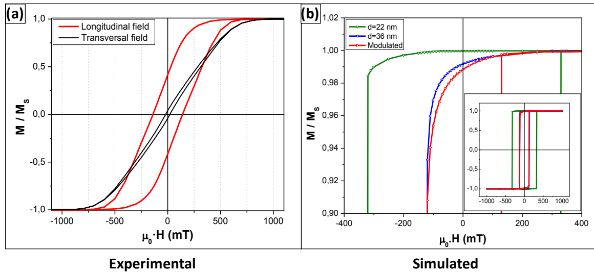
Figure 2.18: Hysteresis loops. (a) VSM hysteresis loops of modulated Fe_{28}Co_{67}Cu_5 nanowires embedded within the Al_2O_3 membrane, with the field applied along the wires' longitudinal axis (red curve) and a transversal direction (black profile). (b) Simulated hysteresis loops of cylindrical homogeneous ( d=22 nm and d=36 nm) and modulated nanowires.
