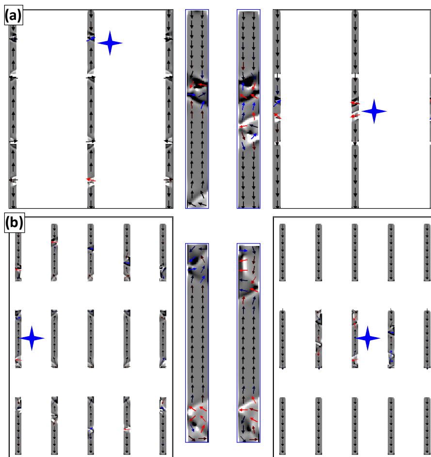
Figure 2.7: Arrays of nanostripes (II). Simulated evolution over time of the reversal process for an applied field of (a) -92 mT and (b) -82 mT, along the easy axis. (a) Longitudinal (transversal) separation distances between stripes are 50 nm (1100 nm). Columns of stripes behave as single structures, with domain walls nucleating at the free ends of the outermost stripes, propagating along them and “jumping” into neighboring nanostructures. (b) Both longitudinal and transversal separations are 500 nm, equivalent to the experimental case. A mixed behavior (see text) suggests that 500 nm is the critical length for the magnetostatic coupling between stripes.
