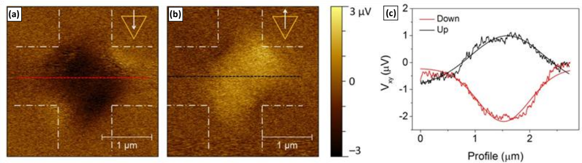
Figure 3.12: Effect of the probe magnetization. SGM mapping of the transverse voltage signal in 0.6- \mu\text{m} wide Hall cross. Images were taken using a homemade probe magnetized (a) downwards and (b) upwards, with the KPFM feedback loop on. The bias current is I_{\text{bias}} = -70 \mu\text{A} . (c) Line profiles obtained along the dashed lines as shown in (a) and (b).
