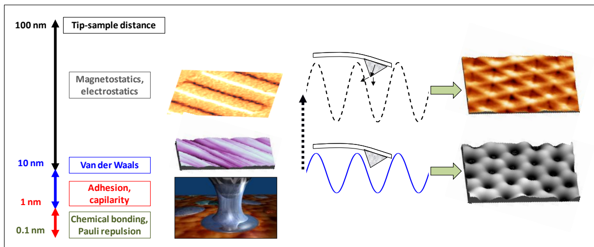
Figure 1.6: Dominant forces as a function of distance. Schematics of the interactions that govern the cantilever dynamics, depending on the separation distance. Typically, van der Waals forces are used to track the topography at distances of few nanometers, from which the cantilever is then lifted by 20-50 nm to obtain the MFM image.
