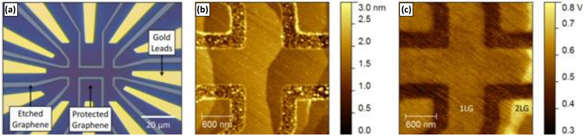
Figure 3.8: Epitaxial graphene devices. (a) Optical image of a 5 \mu\text{m} device showing the gold leads (including gates) and the patterned resist protecting the graphene. (b) Topography and (c) surface potential images of a 0.6- \mu\text{m} wide device.
