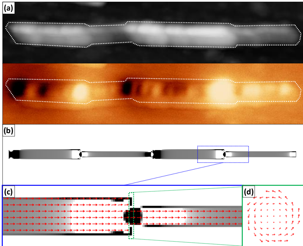
Figure 2.22: The contrast at remanence. (a) High resolution images showing an individual Fe_{27}Co_{68}Cu_5 nanostructure. Strong dark/bright spots are observable in the MFM map. (b) Simulated configuration at remanence for a modulated wire with two thick and two thin parts, equivalent to the experimental case. A single domain state is obtained with large divergence of the magnetic moments at the discontinuities. (c) Zoom in on the blue framed region in (b). Arrows indicate average directions of the simulated spins. (d) Cross section view of the area enclosed by the dashed square line in (c).
