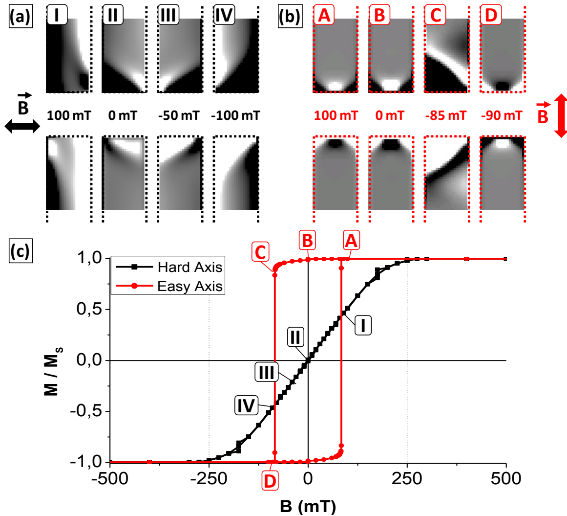
Figure 2.3: Micromagnetic simulations. A single Py nanostripe ( 5 \mu\text{m} \times 100 \text{nm} \times 25 \text{nm} ) was simulated; for clarity reasons, both ends of the same stripe are shown for each case. (a) When large external fields are applied along its hard axis, a transversal dipolar contrast is observed across the stripe (I). For small fields, closure domains are seen at both ends (II)-(III). (b) Closure domains are also formed at the ends, when an external field close to the switching field is applied along the easy axis (C). (c) Simulated hysteresis loops along the easy and hard axis, for the single stripe.
