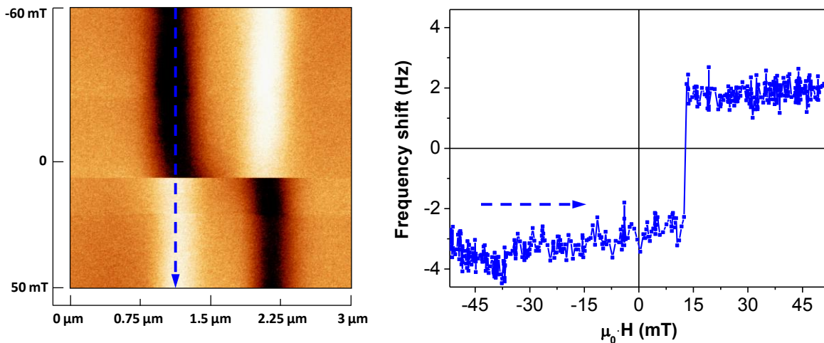
Figure 2.32: Hysteresis loop of a single stripe. Frequency shift 3D mode image performed on the 750 nm wide stripe with the external field applied along its short axis. The field was swept from -60 mT to +50 mT and a switching field value of 12 mT is obtained from the profile plotted on the right.
