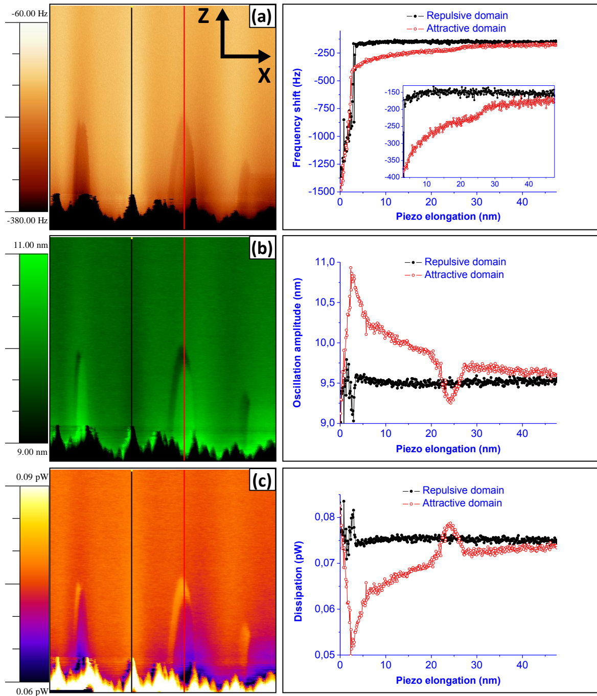
Figure 5.5: 3D modes (II). The tip was again scanned horizontally along 1.5 \mu\text{m} while sweeping the tip-sample distance by 60 \text{ nm} , with an oscillation amplitude of 9 \text{ nm} . A bump and subsequent changes in the (a) frequency shift, (b) amplitude and (c) dissipation images (left column) and profiles in them (right column) are clearly visible.
