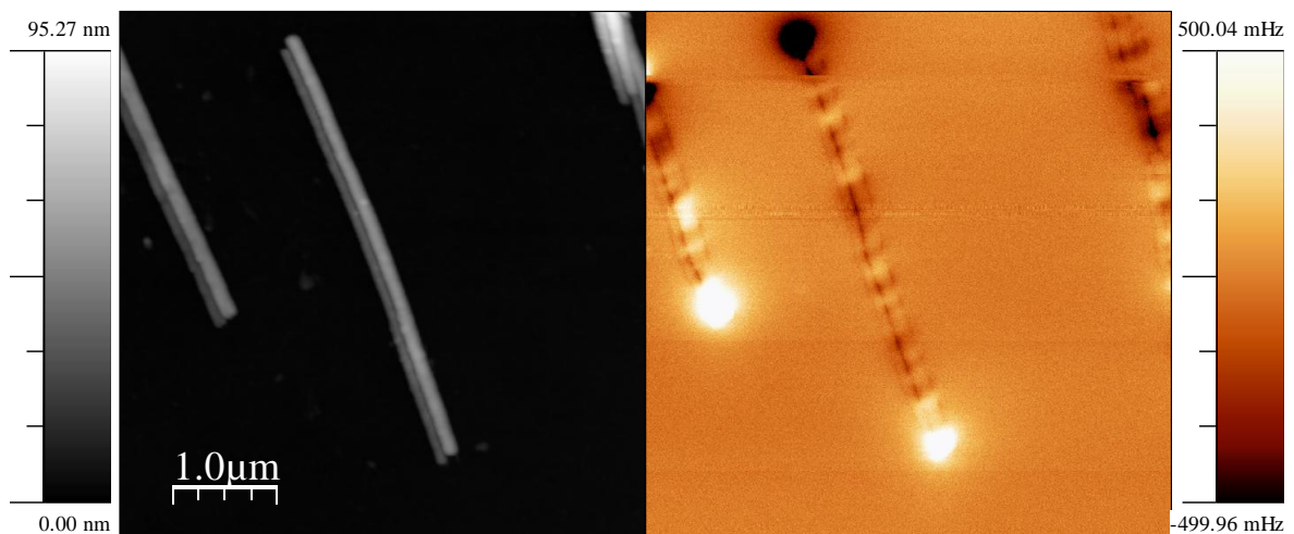
Figure 2.26: Homogeneous \text{Fe}_{28}\text{Co}_{67}\text{Cu}_5 nanowires. Individual nanowire with no modulation in the diameter. The corresponding MFM image shows the wire to be in a single domain state and reflects the same weak contrast along the nanostructure observed for the case of modulated wires.
