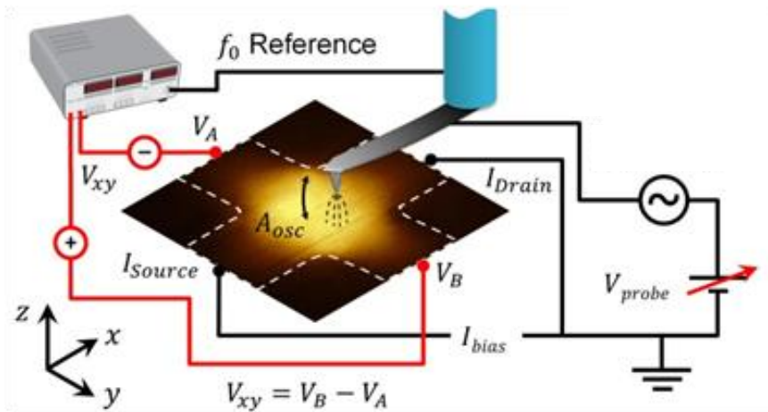
Figure 3.9: Schematics of the measurement set-up used in the experiments. A transversal alternating voltage V_{XY} is induced by the tip in the graphene cross, consequence of Coulomb and Lorentz deviations of electrons, at the oscillation frequency. An external lock-in is used to extract the information.
