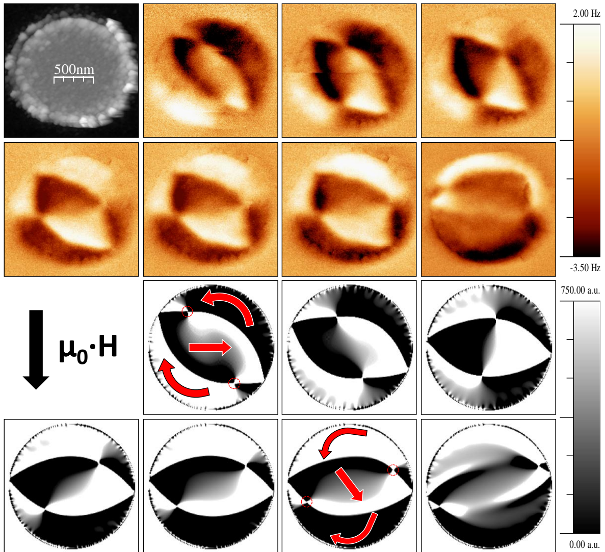
Figure 4.13: The double vortex state. Topography, MFM images and dynamic simulated states of a cobalt dot 1 \mu\text{m} in diameter and 20 \text{ nm} thick, taken under an IP field along the vertical direction. The field sequence in the MFM maps was: -5 \text{ mT} , 0 \text{ mT} , +3 \text{ mT} (upper row), +5 \text{ mT} , +7 \text{ mT} , +10 \text{ mT} and +20 \text{ mT} (lower row), after negative saturation.
