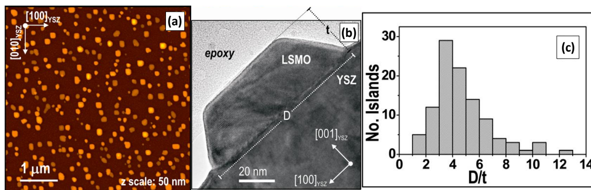
Figure 2.35: The LSMO nanoislands. (a) 5 \times 5 \mu\text{m}^2 topographic image of LSMO nanoislands grown on (001)- YSZ . (b) Cross-sectional TEM image of an LSMO nanoisland with a lateral side to thickness aspect ratio of (D/t) \sim 3.5 ; displaying the typical truncated pyramid geometry. (c) Experimental distribution of the (D/t) aspect ratio.
