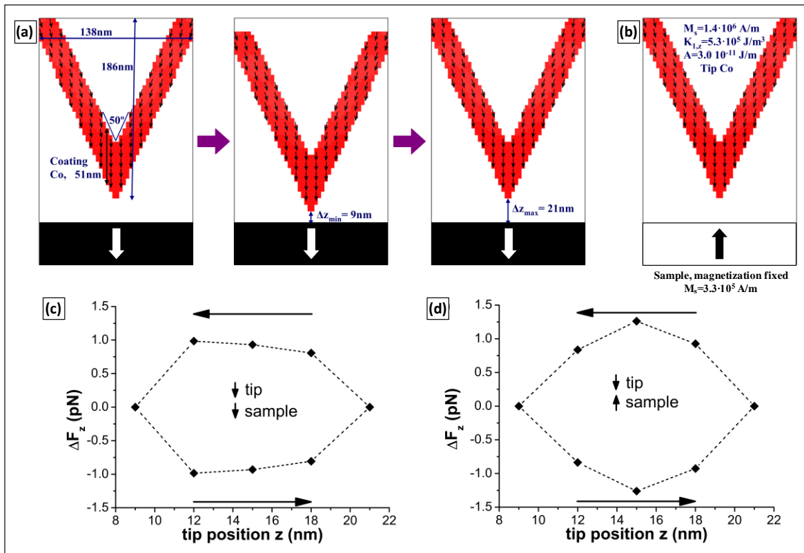
Figure 5.4: Micromagnetic simulations. (a)-(b) Sketch of the tip-sample configuration used in the calculations for (a) attractive and (b) repulsive interactions. (c)-(d) Hysteresis loops in the tip-sample force as function of the separation distance during one oscillation cycle, obtained for the (c) parallel and (d) antiparallel configurations.
