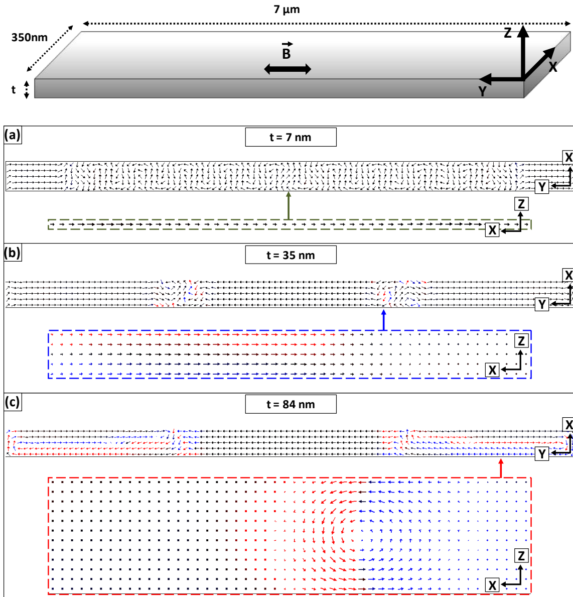
Figure 2.15: The three regimes. Magnetization reversal predicted by micromagnetic simulations for Co stripes 350 wide (X axis) and 7 \mu\text{m} long (Y axis) and variable thickness of (a) 7 nm, (b) 35 nm and (c) 84 nm, with negligible magneto-crystalline anisotropy. Top views (top) and cross sections at the positions highlighted with arrows (bottom) of non-equilibrium steps during the reversal process.
