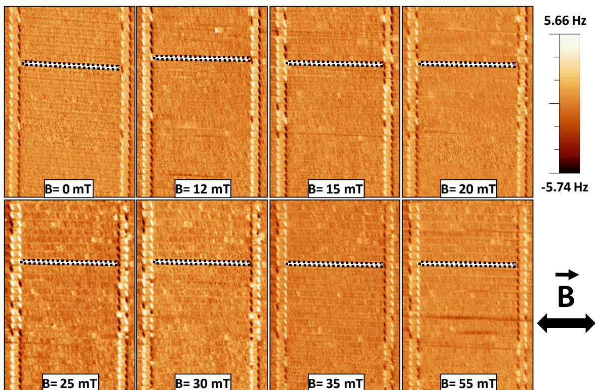
Figure 2.4: The easy axis. Sequence of ( 7 \mu\text{m} \times 13 \mu\text{m} ) MFM images obtained at different magnetic fields applied along the easy-axis of the nanostripes. A particular stripe has been highlighted, as a guide for the eye.
