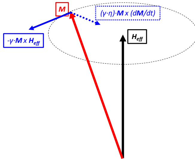
Figure 1.2: LLG equation. Dynamic evolution of the magnetization under the influence of an effective field ( \mathbf{H}_{eff} ), according to the Landau-Lifshitz-Gilbert equation.
