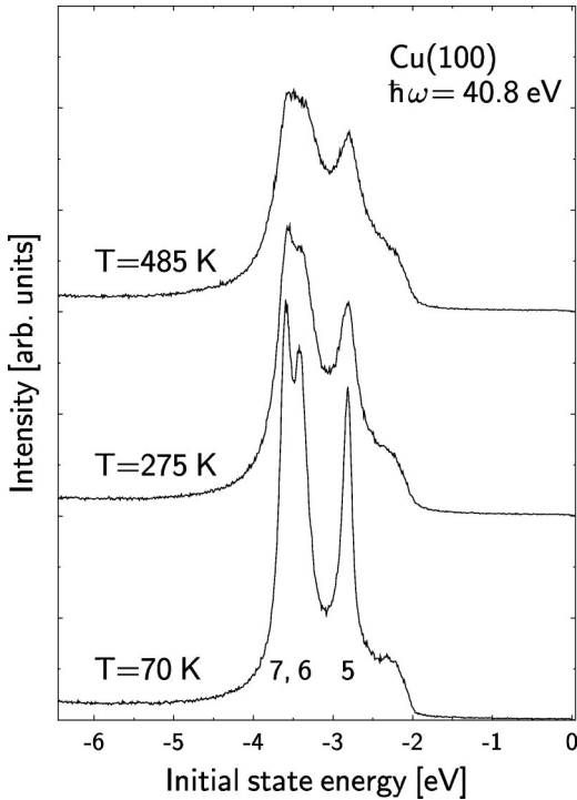
FIG. 4. Normal-emission photoelectron spectra, as obtained at different temperatures from Cu(100) with photons of energy \hbar\omega = 40.8 eV. Peak numbers refer to data collected in Table I.
