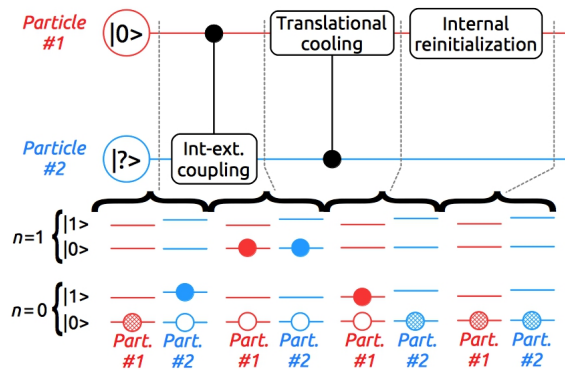
Fig. 5 Cooling protocol via collective modes. The top panel shows the protocol as a diagram in a quantum circuit with the steps discussed in the text indicated as gates. The bottom panel shows the energy states of the system at the start of the process and after each step (dashed vertical lines). The state of a collective mode is indicated by n = 0, 1 , while the internal state of each particle is |0\rangle or |1\rangle as shown. Filled (empty) circles represent the state of each particle when particle #2 is initially internally excited (in its ground state); the hatched circles are states common to both cases: regardless of #2's initial state, the final state always has both #1 and #2 in their internal ground states. Note that the first two steps, even though we act only on one of the particles, involve the collective modes, which we indicate in the top panel by the vertical lines with a bullet.
