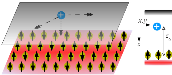
Fig. 7 Ion scanning a lattice of dipoles. (Left) An ion (blue circle) is trapped close to a microfabricated surface trap (grey shaded area) which allows to move it in x, y directions (dashed arrows) above a lattice of dipoles (thick arrows in yellow ovals), and also to shift it closer to the dipoles (dotted arrow). (Right) Cross section showing coordinate system.
