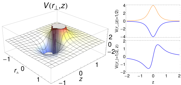
Fig. 2 (Left) Ion-dipole electrostatic energy, V = \mathbf{r}/r^3 , r_{\perp} = \sqrt{x^2 + y^2} . (Right, top) Cuts of V along z = +1/2 (dashed orange line) and z = -1/2 (solid blue). (Right, bottom) Cuts of V along r_{\perp} = \pm 1/2 (both lines overlap).
