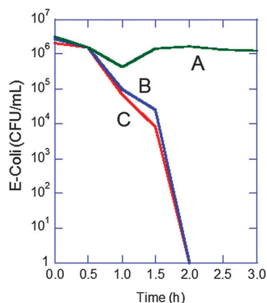
Fig. 41 Change in the bacteria ( E. coli ) concentration with the blue light emission time. A: pristine \text{TiO}_2 , B and C: co-milled with glycine solution and annealed at 500\text{ }^\circ\text{C} . Reprinted with permission from ref. 156. Copyright 2012, Cambridge University Press.
