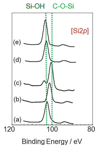
Fig. 38 Si2p XPS spectrum of indomethacin (IM) and silica (S), with milling time in min. (a) IM-50, (b) IM-S30, (c) IM-S180, (d) S30 and (e) S180. Reprinted with permission from ref. 729. Copyright 2004, LAVOISIER SAS.
