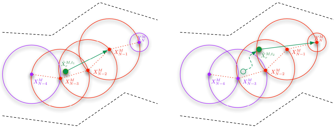
Figure 8: Illustration demonstrating the behavior of the path execution algorithm under normal operating conditions. Waypoints and the circle path are plotted in red when considered by the path execution algorithm, in purple when not. The localization estimate and an arrow signaling the current target are plotted in green. The environment (unknown to the path execution module) is plotted in black. On the left, the circle currently being followed is C_{N-2} , centered on waypoint X_{N-2}^M , and so the current target is X_{N-1}^M . The algorithm considers this circle and its neighbors, in this order: first C_{N-1} , then C_{N-2} and finally C_{N-3} . As the first circle that contains the localization estimate is C_{N-2} , the target does not change. On the right, the robot moves forward and enters circle C_{N-1} , so that the new circle being followed is C_{N-1} and X_N^M becomes the new target.
