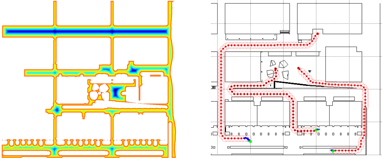
Figure 7: On the left, the cost map for the UPC campus. Warmer tones indicate high costs, white indicates unreachable places. On the right, three sample paths displayed using our simulation environment. Red dots indicate the path computed by the path planning module. Red circles correspond to the circle path, which will be introduced in the following section. Green and blue dots correspond to the localization estimate and mark the starting position for each iteration. Further examples are available in the videos introduced in section 9.
