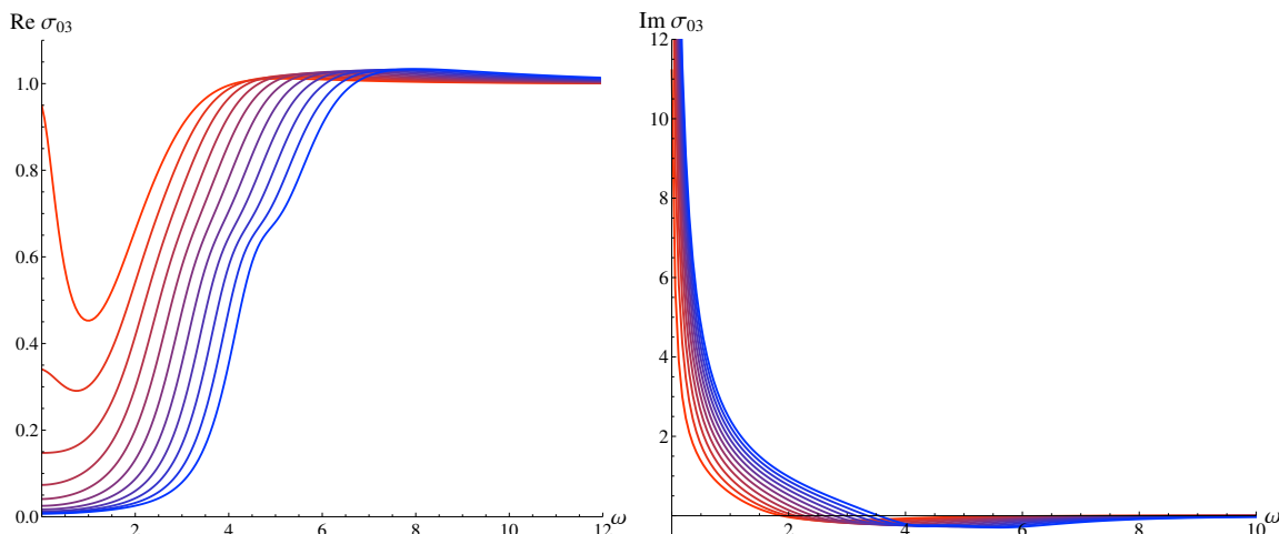
Figure 8. Real (left) and imaginary (right) parts of the conductivity for fixed S_x/\mu = 0.4 . Different lines correspond to different temperatures in the range T = 0.35T_c (blue)– 0.65T_c (red).
