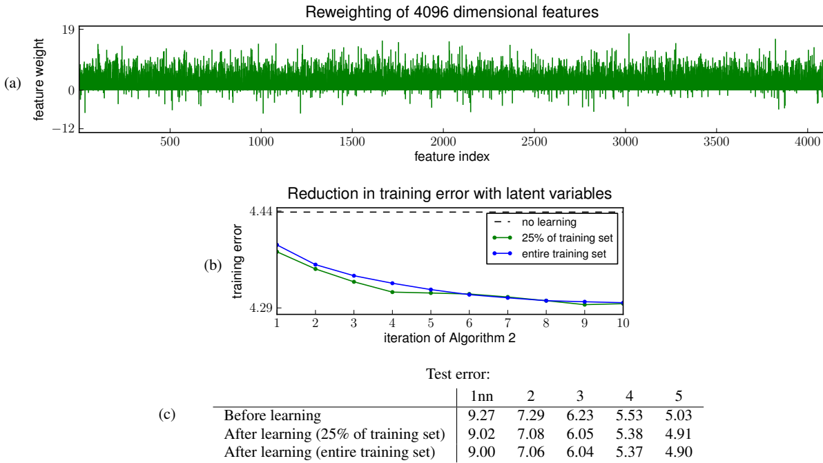
Fig. 3 Results for training with 4096 dimensional features on ImageNet Challenge data. (a) feature weights; (b) reduction in training error during each iteration of Algorithm 2; (c) error for different numbers of nearest-neighbors K (the method was trained to optimize the error for K = 5 ). Results are reported for the best value of \lambda on the validation set (here \lambda = 10^{-6} ).
