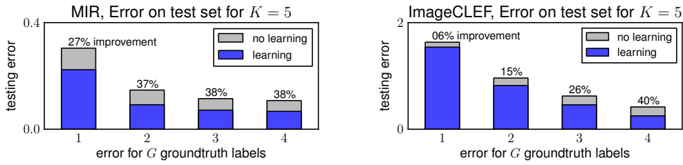
Fig. 8 Improvement of learning over non-learning for the MIR and ImageCLEF taxonomies as the number of groundtruth labels G increases. ‘Testing error’ refers to the average loss across all images in the test set. The plots are annotated to show the percentage improvement of learning over non-learning. All results are reported for the best value of \lambda on the validation set. Note that the final two bars for the MIR dataset are almost identical simply due to the fact that few images have as many as four labels owing to the small size of the label vocabulary.
