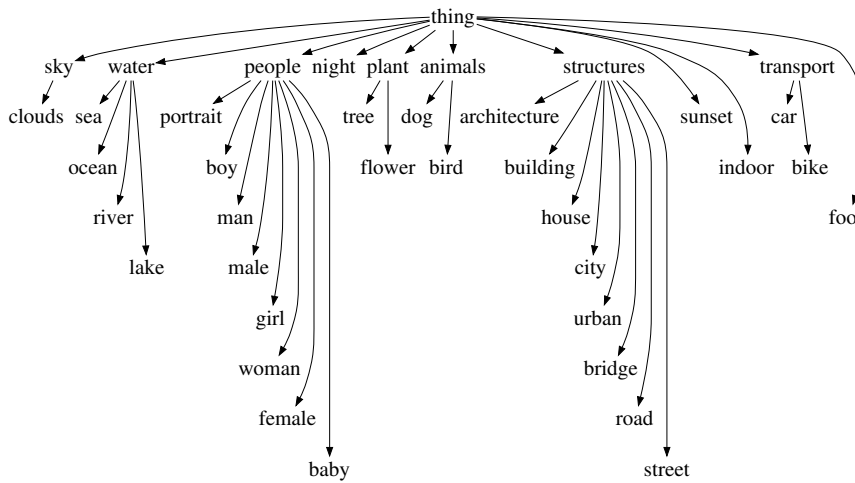
Fig. 4 The MIR taxonomy. Twenty-four of the tree’s nodes are the possible labels for each image.
