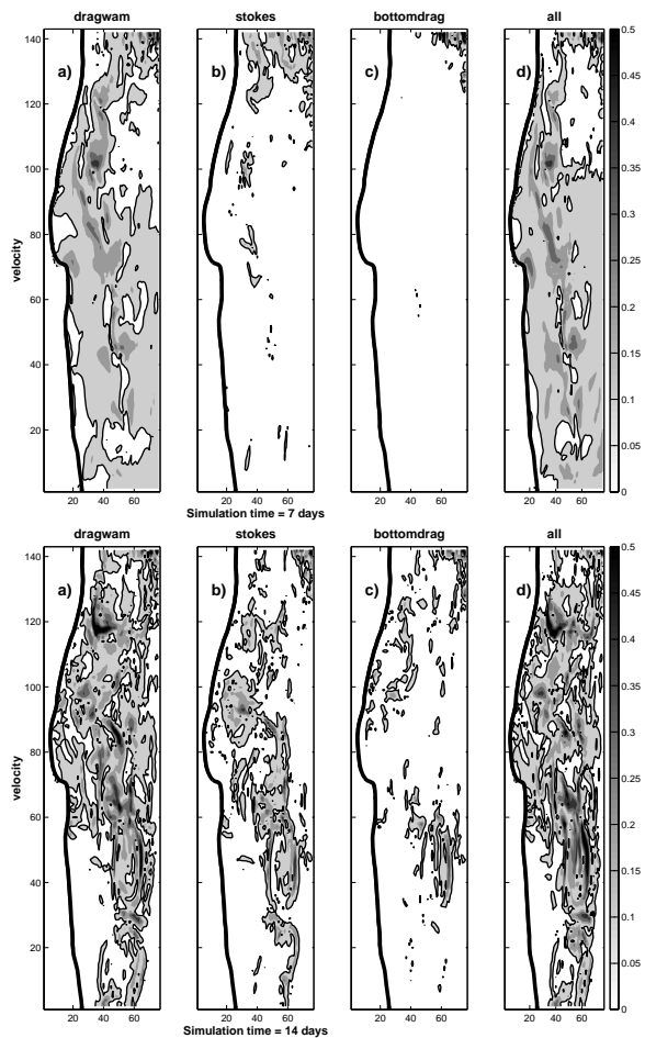
Fig. 7. The same than Fig. 5 but for the velocity field. The contours interval is 10 \text{ cm/s kg/m}^3 . The thick line shows the 10 \text{ cm/s} difference.
