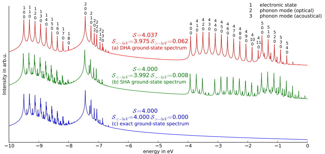
FIG. 3. Calculated Photoelectron spectra for Trans-Polyacetylene: (a) The ground-state spectrum in double-harmonic approximation (DHA), (b) the ground-state spectrum in single-harmonic approximation (SHA) (c) the exact ground-state spectrum from the full-quantum calculation. With S we refer to the value of the sum rule for the spectral function as defined in Eq. 17. For a complete set of states this corresponds to the total number of electrons. Restricted summations of the sum rule in the energy range above -5 eV and below -5 eV are given by S_{>-5\text{eV}} and S_{<-5\text{eV}} , respectively.
