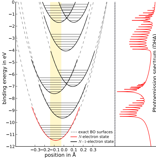
FIG. 2. Exact Born-Oppenheimer surfaces and harmonic approximation for a Trans-Polyacetylene oligomer: In the panel on the left-hand side, an one-dimensional cut along the optical axis of the exact potential energy surfaces is shown in dashed lines. The harmonic approximations to the exact BO surfaces are shown in solid lines, where black lines refer to N - 1 electron states and the red line corresponds to the N -electron ground state. In the panel on the right hand side, the corresponding photoelectron spectrum in double-harmonic approximation is shown.
