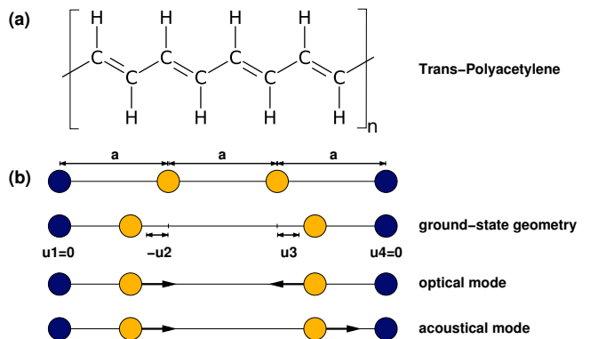
FIG. 1. (a) Chemical structure of Trans-Polyacetylene. (b) Model system for SSH-chain: four Trans-Polyacetylene oligomers with clamped ends. The coordinates u_j describe the shift of the oligomers with respect to a perfectly periodic arrangement of lattice spacing a . Both, in the exact Born-Oppenheimer and in the exact correlated ground state, the chain favors a dimerized arrangement. Also shown are the optical and acoustical phonon modes of the chain.
