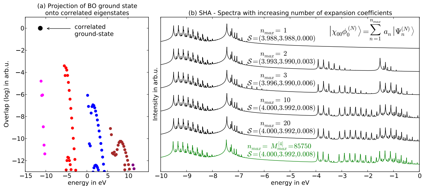
FIG. 4. Non-adiabatic contribution to the BO ground state of the Trans-Polyacetylene chain: (a) Projection of the BO ground state onto correlated eigenstates. (b) SHA spectra depending on expansion coefficients. Here, S = (S, S_{<-5\text{eV}}, S_{>-5\text{eV}}) , as in Fig. 3.
