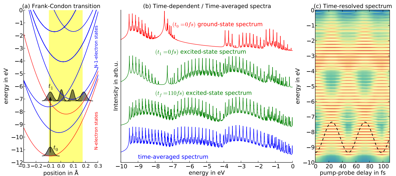
FIG. 5. (a) Illustration of Frank-Condon transition: The excited N -electron initial state propagates on the Born-Oppenheimer surface of the first excited electronic state. N -electron potential-energy surfaces are shown in red, N - 1 -electron potential-energy surfaces in blue. The oscillation spread of the center of the wavepacket is indicated by a yellow background. The different wavepacket shapes indicate the squeezing of the vibronic state. (b) Spectra at different time-steps (the first spectrum at t_0 corresponds to spectrum (b) in Fig. 3), (c) All obtained spectra plotted time-resolved, the color code refers to high intensity in red and low intensity in blue color. The dashed black line shows the motion of the center of the nuclear wavepacket as function of pump-probe delay. The color code refers to high intensity in red and low intensity in blue color.
