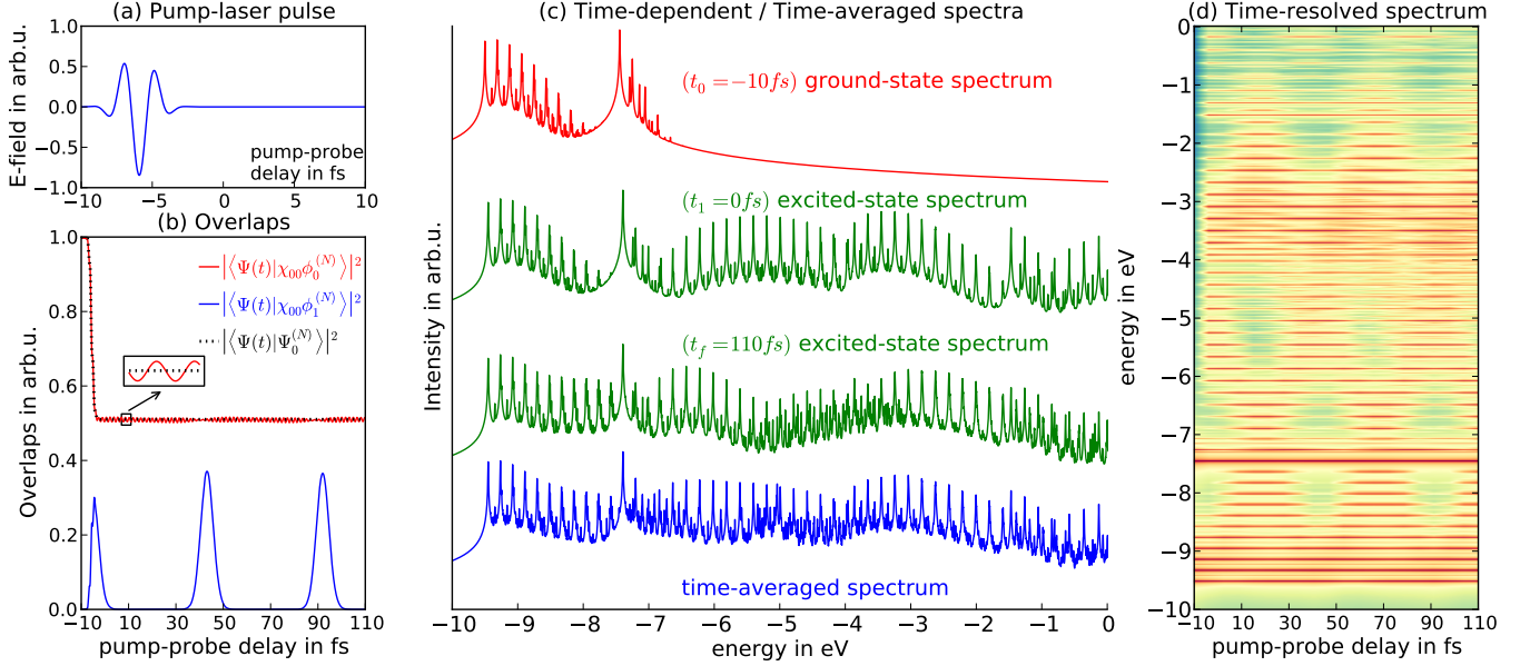
FIG. 6. Time-dependent pump-probe photoelectron spectroscopy: (a) Amplitude of laser-pulse as given in Eq. 9, (b) overlaps of time-evolved state with electronic ground and first excited Born-Oppenheimer states and the exact correlated ground state, (c) spectra at different time-steps (the first spectrum at t_0 corresponds to spectrum (c) in Fig. 3), (d) all obtained spectra plotted time-resolved, the color code refers to high intensity in red and low intensity in blue color.
