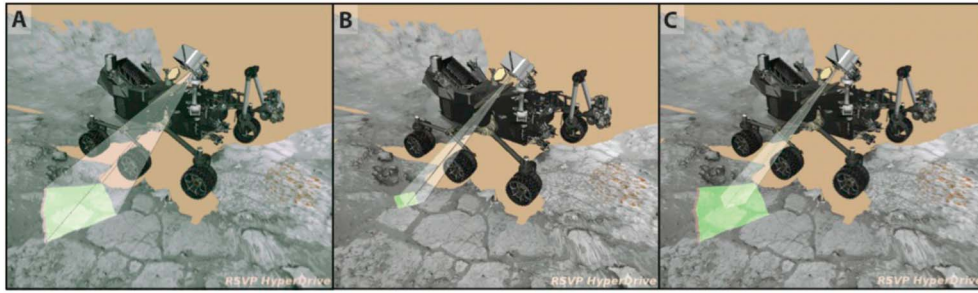
Figure 2. RSVP hyperdrive modeling of clast survey image positions. (a) Position of M-34 image footprint. (b) Position of M-100 image footprint. (c) Combined M-34 and M-100 image footprints. Differences in sighting between M-34 and M-100 images, combined with the angle of viewing for the clast survey results in location of the M-100 image frame near the lower right-hand side of the M-100 image frame.
