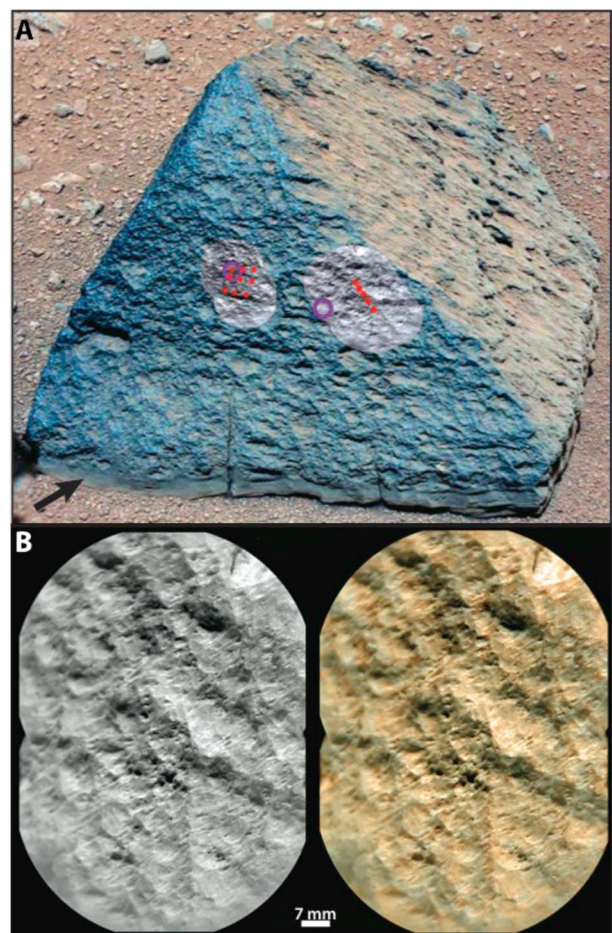
Figure 12. Jake Matije vic ventifact. (a) Mastcam 100 image with superposed RMI mosaics shown in gray scale; red dots are the location of LIBS spots. (b) The rightmost RMI mosaic is enlarged in at left, with merged Mastcam color at right [Le Mouélic et al. , 2013]. Jake Matije vic has the most prominent abrasion textures seen in the first 100 sols, with a distinct keel at its crest (arrow), penetrating flutes, elongated pits, lineations, and a basal sill.
