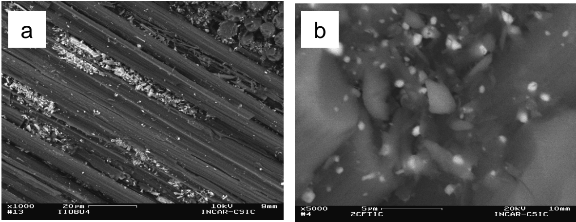
Figure 3.- SEM micrographs of carbon fibre preform after thermal decomposition of TBO.
