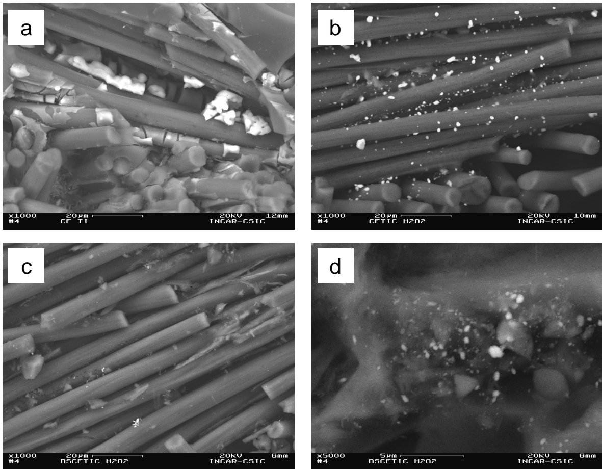
Figure 4.- SEM micrographs of: a) carbon fibre preform after decomposition of TBO with H 2 O 2 ; b) doped preform after treatment at 1000°C; c) and d) carbonised composite.
