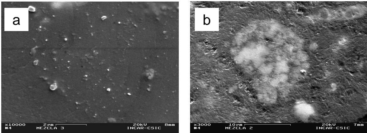
Figure 1.- SEM micrographs of doped precursors: a) AR-TBO-3 and b) AR-TBO-15.
