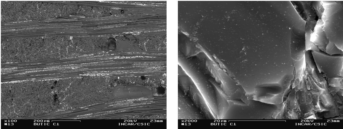
Figure 5.- SEM micrographs of Ti-doped composite obtained by combination of doping methods.
