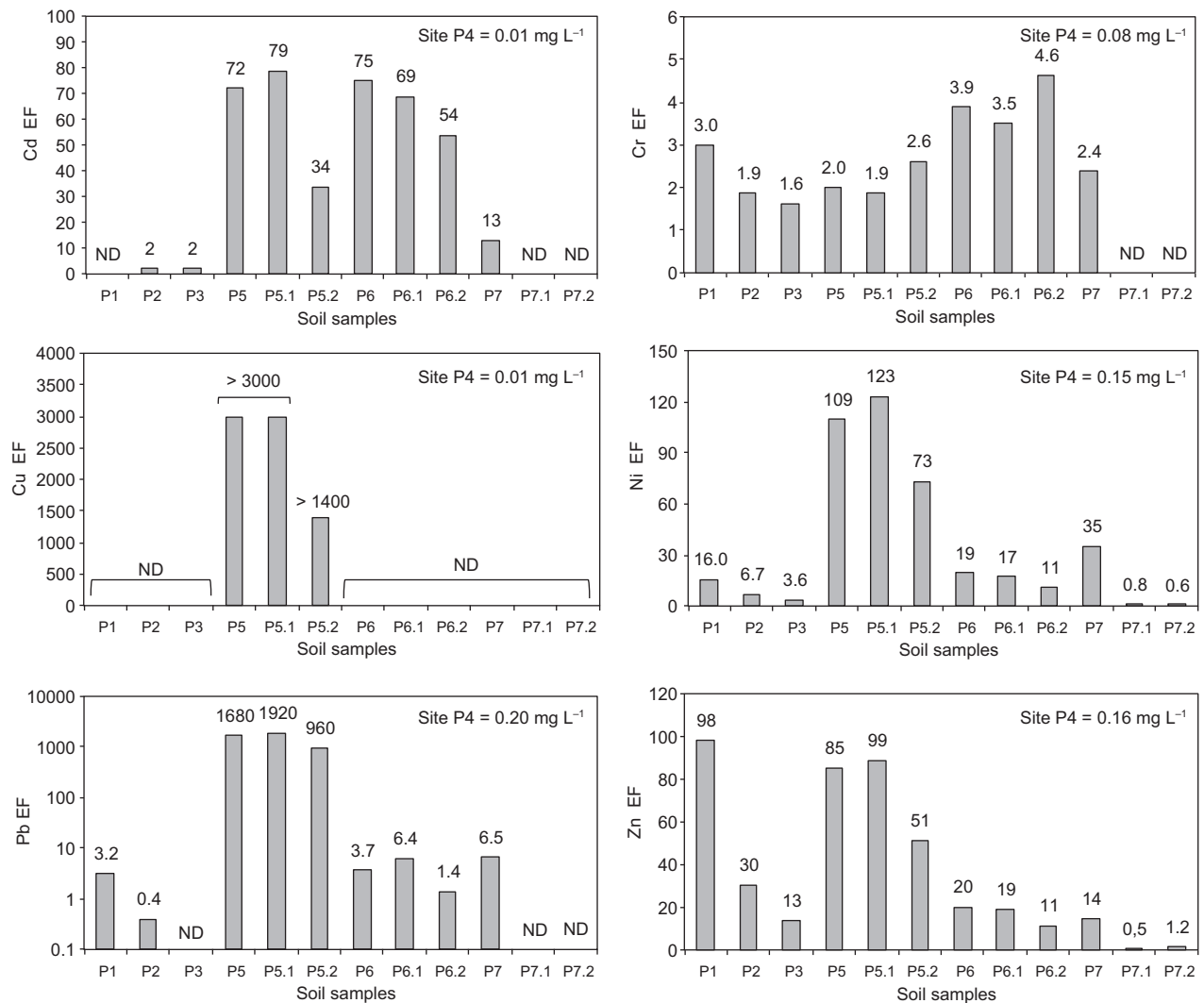
Fig. 3. Metal enrichment factors (EF) in relation to a reference site (site P4) for the average TCLP values reported in figure 3. ND denotes that EF was not determined since the analyzed sample presented a result below the analytical detection limit. Note that Cu EFs from site 5 samples are related to a control site concentration below the analytical detection limit.
