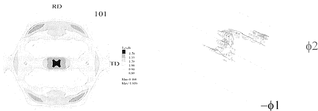
Fig. 11. The pole figure (101) and the ODF of the deposit (phase \text{InSn}_\beta ). A non-stirred solution ( \omega = 0 rad/s)
