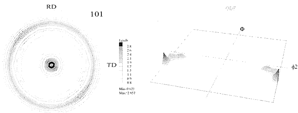
Fig. 10. The pole figure (101) and the ODF (axial symmetry) of the deposit (phase \text{InSn}_\beta ). A stirred solution ( \omega = 14 rad/s)
