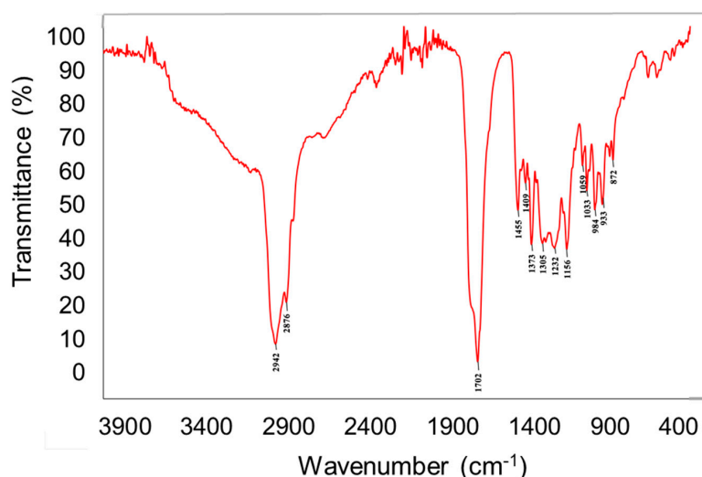
Figure 1. FTIR spectra of Heterobasidion annosum extract.
