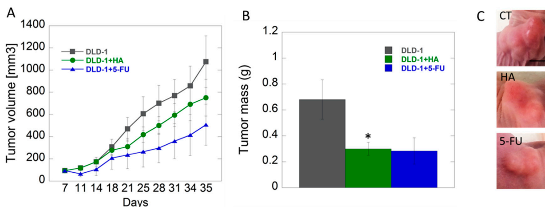
Figure 4. Analysis of tumor volume (panel A) and tumor mass (panel B) changes in study groups (control–DLD-1, HA-1 mg/kg body weight, DLD-1+5-FU); example images of tumors (C), scale bar = 0.5 cm * p < 0.05 vs. control.
