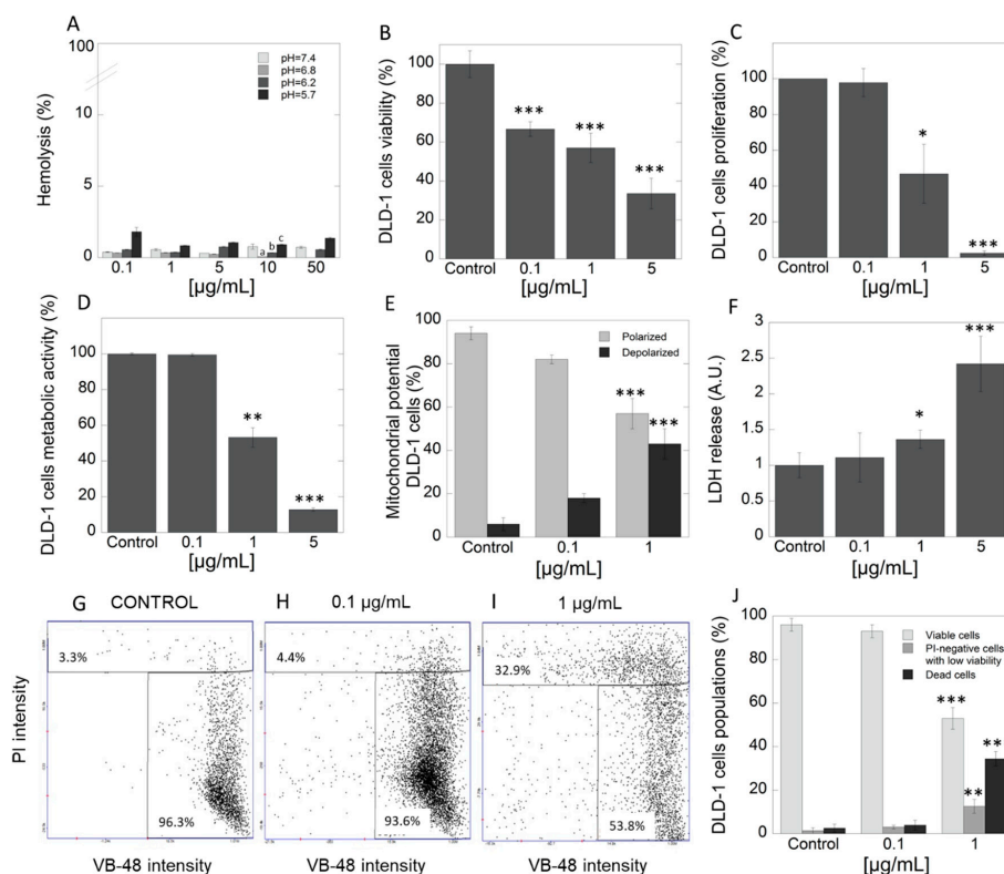
Figure 2. Hemocompatibility and cytotoxicity of Heterobasidion annosum (HA) extract against DLD-1 cells. Panel A shows high compatibility of HA extract against representative of host cells—RBC cells. The ability to decrease viability (panel B) and proliferation (panel C) of DLD-1 colorectal cancer cells after treatment with HA extract at different concentration range 0.1–5 \mu\text{g/mL} . Pleiotropic mode of action of HA extract—reduction of metabolic activity (D), increasing number of depolarized cells (E), and leakage of LDH from the treated cells (F). The distribution of thiol levels in DLD-1 cells after treatment by HA extract—fluorescence intensity scatters (G-control, H-0.1 \mu\text{g/mL} and I-1 \mu\text{g/mL} ) and column plot (J). PI—propidium iodide, VB-48—VitaBright-48 iodide; Statistical significance: (pH = 7.4) vs. (pH = 6.8) a p < 0.01 ; (pH = 6.8) vs. (pH = 6.2) b p < 0.01 ; (pH = 6.8) vs. (pH = 5.4) c p < 0.01 (panel A); * p < 0.05 vs. control, ** p < 0.01 vs. control; *** p < 0.001 vs. control.
