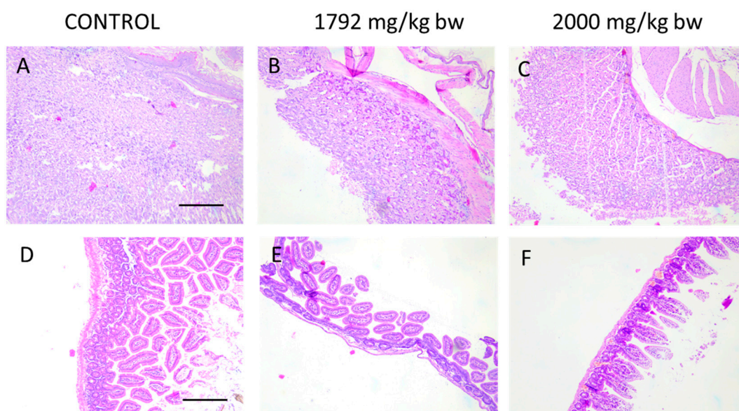
Figure 5. Histological images of stomach (A–C) and intestine (D–F) showing no pathological changes in animal receiving the highest doses of HA extract in acute toxicity study. Magnification 100 \times .
