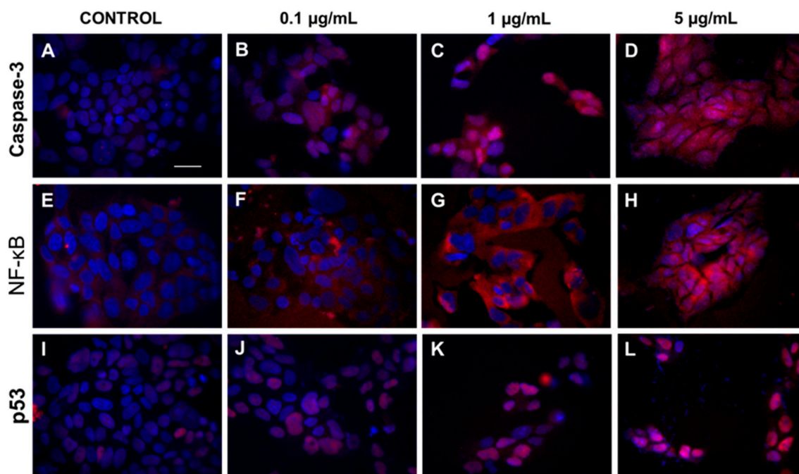
Figure 3. The cytoplasmatic and nucleus level of caspase-3, NF- \kappa B, and p53 in DLD-1 cell line after HA extract application. Panels (A–D) show expression of caspase 3 after treatment of DLD-1 by different concentrations of HA extract (0.1–5 \mu g/mL). Increasing expression of NF- \kappa B and p53 protein after addition of HA extract at different concentration range 0.1–5 \mu g/mL are showed at panels (E–H) and (I–L), respectively. Magnification 400 \times , Scale bar = 20 \mu m.
