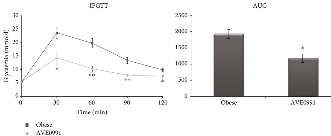
FIGURE 1: Intraperitoneal glucose tolerance test (IPGTT) evaluated in control obese Zucker rats ( n = 6 ) and in obese Zucker rats receiving AVE0991 ( n = 5 ) via osmotic minipumps for two weeks. AUC: area under curve. Data are presented as mean \pm S.E.M. and were analysed using Student's t -test, * p < 0.05 ; ** p < 0.01 .
