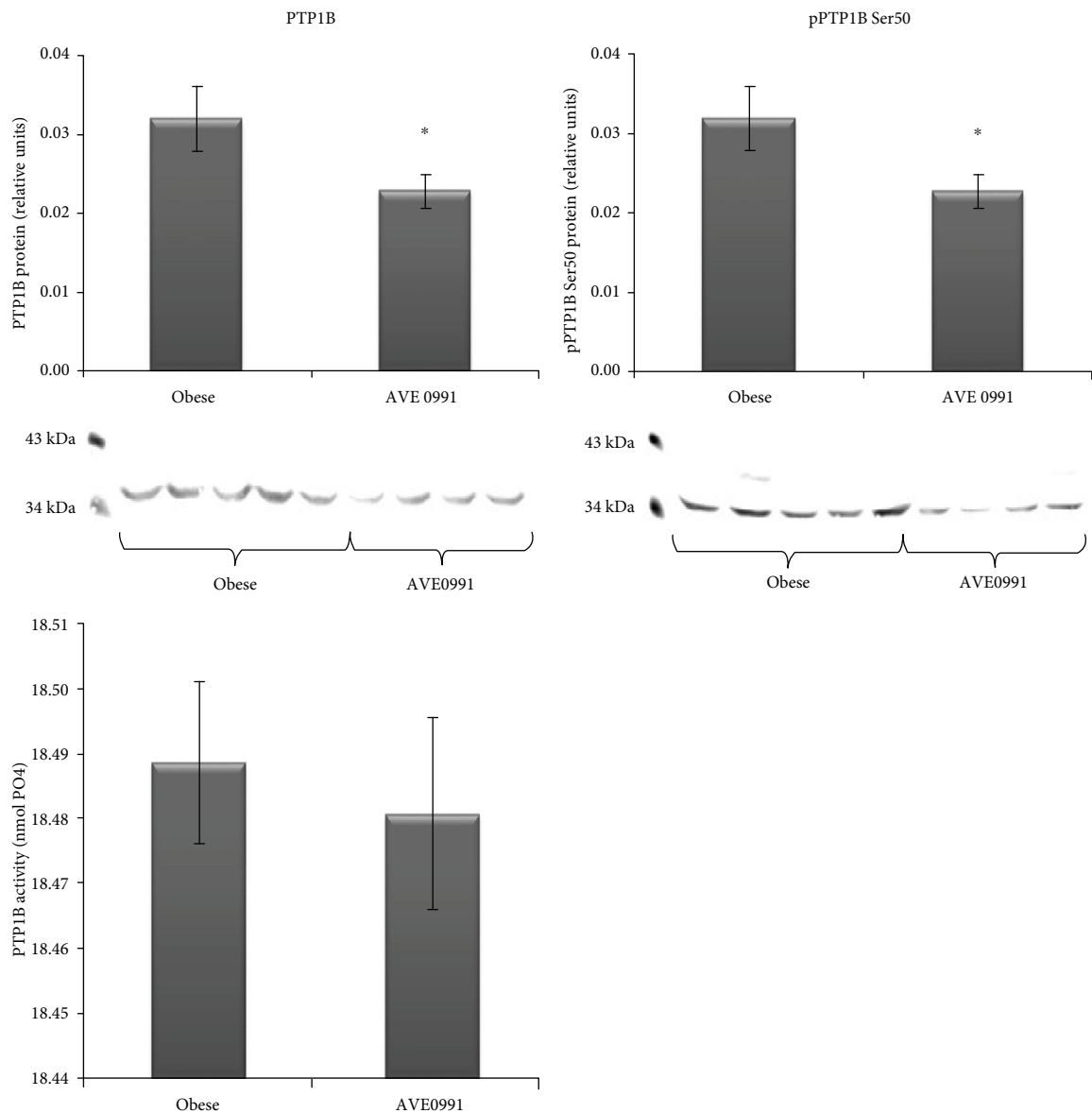
FIGURE 9: Protein tyrosine phosphatase 1B (PTP1B) in the skeletal muscle of obese Zucker rats. Protein content of total protein tyrosine phosphatase 1B (PTP1B), phosphorylated PTP1B at Ser50 with representative Western blots, and PTP1B activity in musculus quadriceps of control obese Zucker rats and in obese Zucker rats receiving AVE0991 via osmotic minipumps for two weeks. The amount of protein was quantified by Western blot method, and PTP1B activity was measured using commercially available colorimetric assay kit. The signal intensities of the proteins of interest were normalized to the sample's total protein content stained with Coomassie Brilliant Blue. Data are presented as mean ± S.E.M. Results were analysed by Student's t -test, * p < 0.05; ** p < 0.01; *** p < 0.001.
