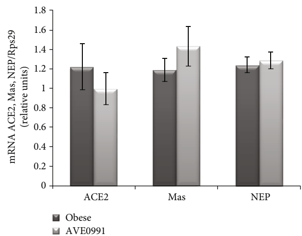
FIGURE 3: Alternative RAS pathway components in the skeletal muscle of obese Zucker rats. Gene expression of angiotensin-converting enzyme2 (ACE2), Mas receptor, and neutral endopeptidase (NEP) in musculus quadriceps of control obese Zucker rats and in obese Zucker rats receiving AVE0991 via osmotic minipumps for two weeks, determined by real-time PCR. Data were normalized to the gene expression of 40S ribosomal protein S29 (Rps29) whose expression was not altered by the treatment. Data presented as mean \pm S.E.M. were analysed by Student's t -test.
