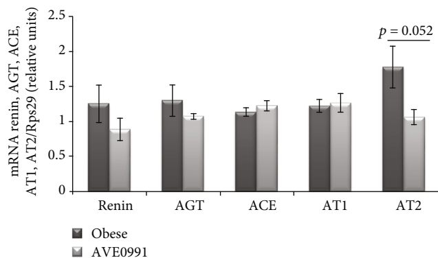
FIGURE 2: Classical RAS pathway components in the skeletal muscle of obese Zucker rats. Gene expression of renin, angiotensinogen (AGT), angiotensin-converting enzyme (ACE), angiotensin II type 1 receptor (AT1), and angiotensin II type 2 receptor (AT2) in musculus quadriceps of control obese Zucker rats and in obese Zucker rats receiving AVE0991 via osmotic minipumps for two weeks, determined by real-time PCR. Data were normalized to the gene expression of 40S ribosomal protein S29 (Rps29) whose expression was not altered by the treatment. Data presented as mean \pm S.E.M. were analysed by Student's t -test.
