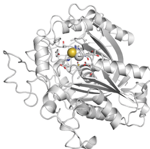
Figure 1. The central KS domain of the loading/condensing region (SAT-KS-MAT) of C. uncialis polyketide synthase. The active site is depicted with Cys547 shown with spheres and other residues are shown with a balls and sticks representation.
