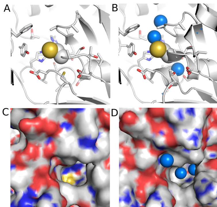
Figure 4. Comparison of C. uncialis (A and C) and C. nicotianae (B and D) active sites in KS domains.
