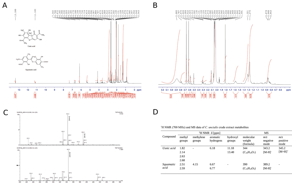
Figure 2. 1 H NMR and MS analysis of Cladonia ucialis acetone extract.
