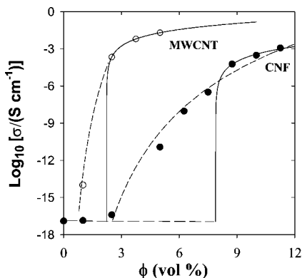
Figure 10. Logarithm of the electrical conductivity versus nanoadditive volume concentration for the CNF (●) and MWCNT (○) nanocomposites. The continuous line is the fitting of eq 5 according to percolation theory. The dashed lines are the predictions according to tunneling conduction.
