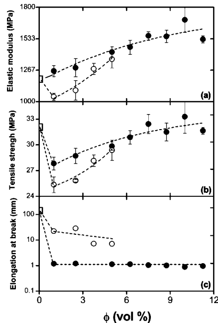
Figure 8. Summary of mechanical properties of HDPE nanocomposites with HDPE ( \square ); CNF ( \bullet ) and MWCNT ( \circ ): (a) elastic modulus, (b) tensile strength and (c) elongation at break. The dashed lines are a guide for the eye.
