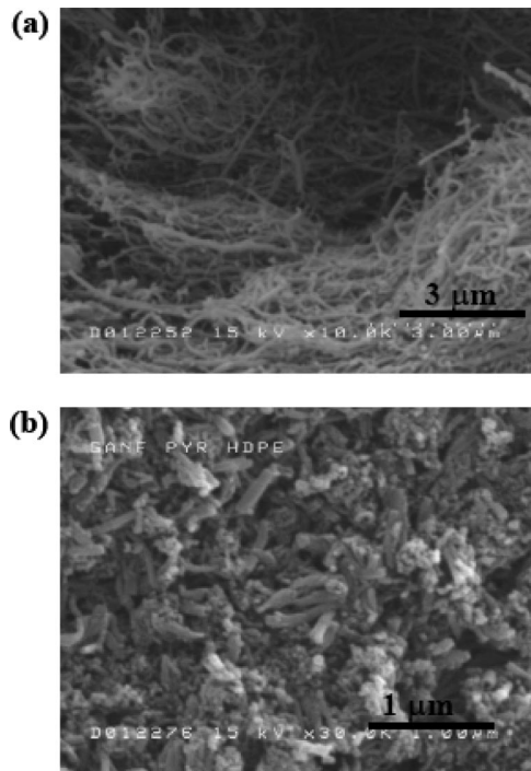
Figure 7. SEM micrographies of (a) MWCNT and (b) CNF after extraction from the nanocomposites. The scale bars are indicated on the bottom right.
