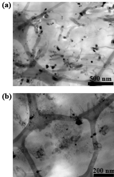
Figure 6. TEM micrographies of HDPE nanocomposites with (a) MWCNT and (b) CNF. The scale bars are indicated on the right. The background honeycomb-like structure is due to the TEM grid.
