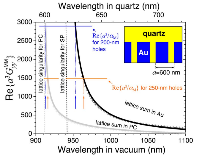
FIG. 18. (Color online) Lattice sums and lattice resonances in a square array of holes drilled in gold vs a perfect conductor. The real part of the exact lattice sum for interaction of parallel magnetic ( M ) dipoles is shown for gold (black curve) and for a perfect conductor (PC, gray curve), as compared to analytical approximate expressions (symbols). The Rayleigh condition for a period a=600 nm is indicated by gray and black vertical dashed lines for light in the dielectric ( \lambda/n=a ) and for surface plasmons ( \lambda_{\text{SP}}=a ), respectively. Changes in the inverse magnetic polarizability of circular holes of different size [horizontal lines, as obtained from Fig. 7(b) (see footnote 9)], lead to different wavelengths of the lattice surface modes, as indicated by vertical arrows for the condition that the real part of the denominator of Eq. (3) be zero.
