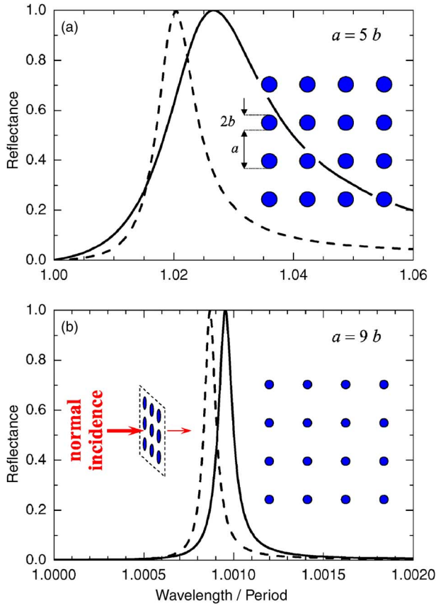
FIG. 3. (Color online) Reflectance spectra of square arrays of perfectly conducting thin circular disks. The wavelength \lambda is normalized to the lattice constant a . The disks radius is (a) b = a/5 and (b) b = a/9 . Light is impinging normal to the array and 100% reflection is observed in these two cases at the maximum. Solid curves, full numerical results. Dashed curves, analytical model for |r|^2 [Eq. (11)].
