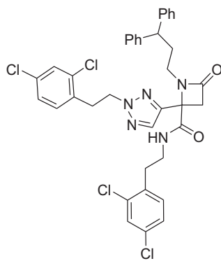
Fig. 2. Compound 9.
