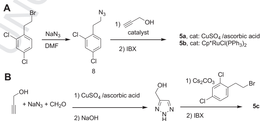
Scheme 2. Syntheses of aldehydes 5a-c .
