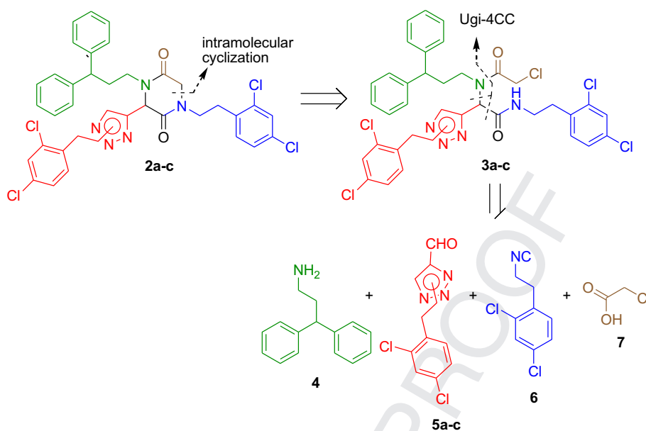
Scheme 1. Retrosynthesis of 2a-c comprising an Ugi-4CC reaction followed by an intramolecular cyclization.
