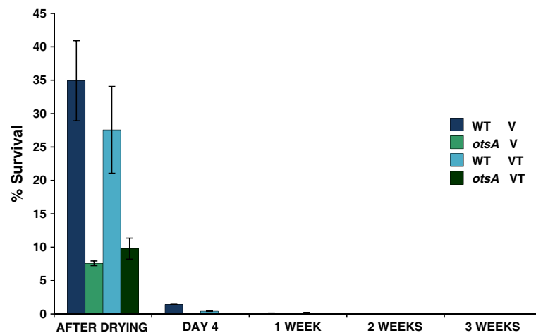
Figure 6 Survival of R. etli strains after vacuum-drying and subsequent storage at 28°C. R. etli wild-type and otsA mutant were cultured at 28°C in minimal medium B' with 0.2 M NaCl until they reached early stationary phase: Desiccation was performed as described in Methods, using vacuum or vacuum + temperature conditions. After drying, samples were sealed and stored at 28°C. Viability was measured before (taken as 100% survival), just after drying, and after 4 days, 1, 2 and 3 weeks storage, and expressed as percentage of viable cells. Error bars indicate standard deviations.
