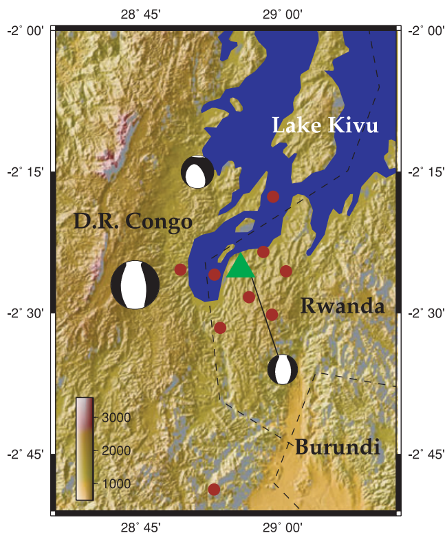
Figure 5. Focal mechanisms from the teleseismic data (this study) for the mainshock (2008 February 03, 7:34:13) and for two aftershocks (northern is 2008 February 14, 2:07:47, southern is 2008 February 03, 10:56:10). Red dots show the USGS National Earthquake Information Centre's locations for earthquakes within a month of the mainshock. The green triangle shows the location of the rupture fault obtained from the geodetic inversion (this study).
