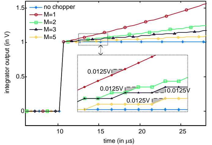
Fig. 4. First integrator impulse response for different chopper frequencies.
