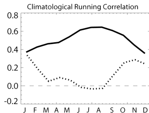
Figure 4. Climatology of the 60 day (120 day) running correlation between the SVD time series for SST and wind stress for two frequency bands. The solid (dotted) line is for the 1–30 day -1 ([30, \infty ] day -1 ) frequency band. Correlation above 0.2 are significant at the level \sigma = 95\% .
