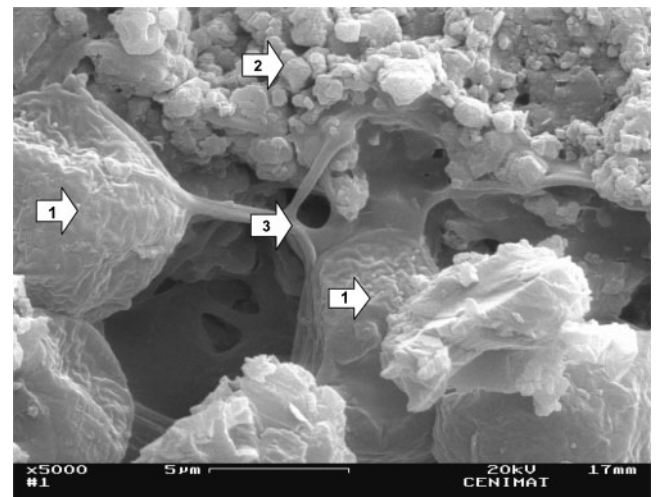
Fig. 9. SEM image showing green algae cells (arrow 1) adhered to a limestone surface (arrow 2) embedded in matrix of extracellular polymeric substances (arrow 3). Scale bar, 5 μm.
