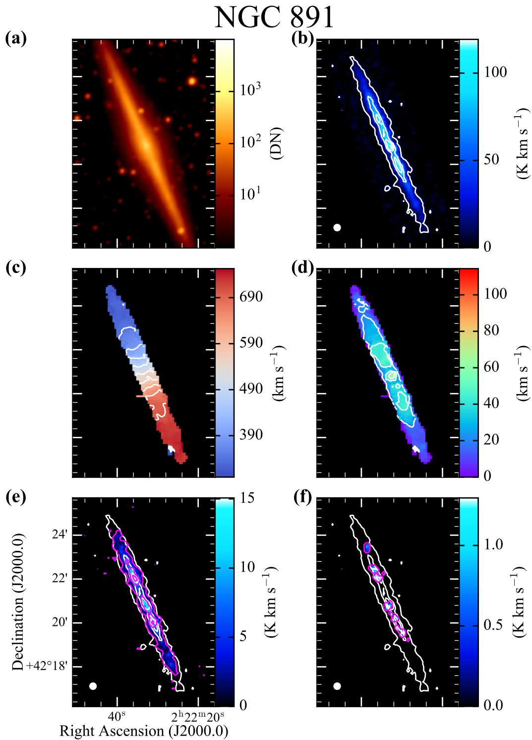
Fig. 12. NGC 891. (a) Background-subtracted WISE 3.4\mu\text{m} image. (b) Integrated intensity of ^{12}\text{CO} ( J = 1 - 0 ). The contours are plotted at 5%, 40%, and 60% of the maximum intensity of 152.45 \text{ K km s}^{-1} . (c) First-degree moment map of ^{12}\text{CO} . The contours are in 45 \text{ km s}^{-1} steps. (d) Second-degree moment map of ^{12}\text{CO} with the contours in steps of 20 \text{ km s}^{-1} . (e) Integrated intensity of ^{13}\text{CO} ( J = 1 - 0 ). The white contours are the same as the panel (b). The magenta contours are plotted at 5%, 45% and 85% of the maximum intensity of 16.53 \text{ K km s}^{-1} in ^{13}\text{CO} . (f) Integrated intensity of \text{C}^{18}\text{O} ( J = 1 - 0 ). White contours are the same as the panel (b). The magenta contours are plotted at 5% of the maximum intensity of 2.26 \text{ K km s}^{-1} in \text{C}^{18}\text{O} . The OTF beam size is indicated as a white filled circle in the bottom-left corner in panel (b), (e), and (f).
