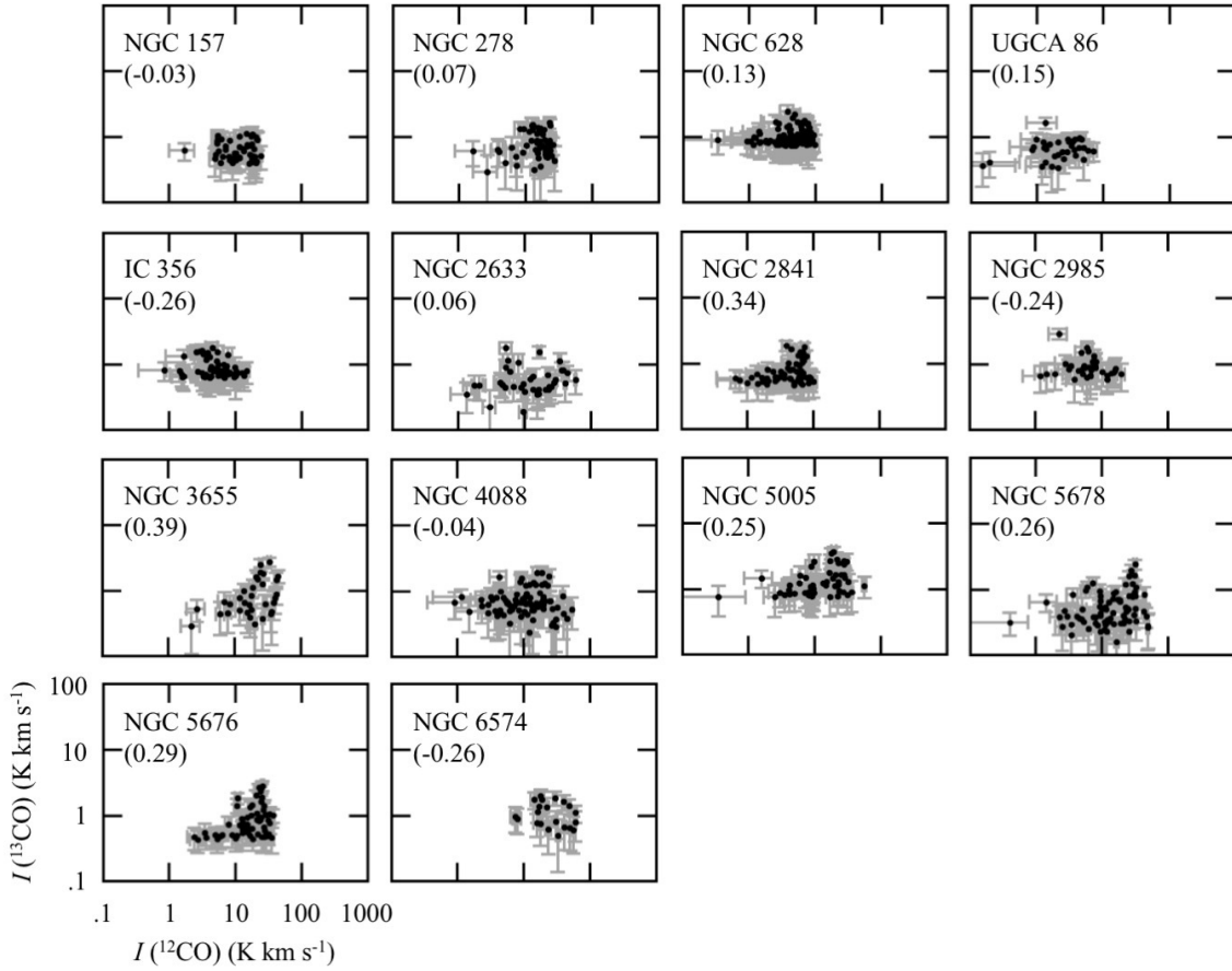
Fig. 19. Same as figure 17, but for galaxies with |\rho_{I(12CO), I(13CO)}| < 0.4 .
