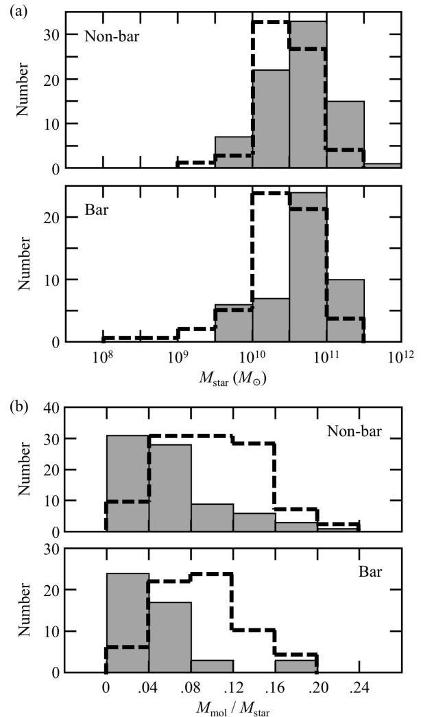
Fig. 28. (a) Histograms of the total stellar mass M_{\text{star}} for the non-barred and barred galaxies in the EDGE sample (Bolatto et al. 2017). The dashed line indicates the COMING results shown in figure 26 for SA and SAB + SB. (b) Same as (a), but for M_{\text{mol}}/M_{\text{star}} . The dashed line indicates the COMING results shown in figure 27 for SA and SAB + SB. The COMING results are normalized for the peak to correspond to that of the EDGE results, and the data with uncertainty or upper/lower limit data are not used.
