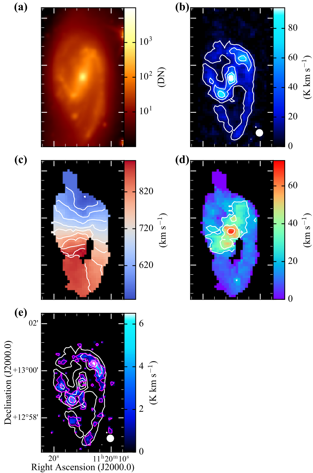
Fig. 13. Same as figure 12, but for NGC3627. The contours are plotted at 10%, 30%, 55%, and 80% of the maximum intensity of 109.87 K km s -1 in (b) and (e) ( white ), in steps of 40 km s -1 in (c), in steps of 20 km s -1 in (d), and at 10%, 45%, and 80% of the maximum intensity of 7.88 K km s -1 in (e) ( magenta ).
