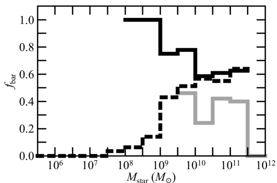
Fig. 29. Bar fraction f_{\text{bar}} of the COMING sample as a function of the stellar mass M_{\text{star}} ( black solid ). The data with a large uncertainty or the upper limit data are not used. The fractions of the EDGE sample (Bolatto et al. 2017) ( gray solid ) and S 4 G (Díaz-García et al. 2016) ( black dashed ) are shown.
