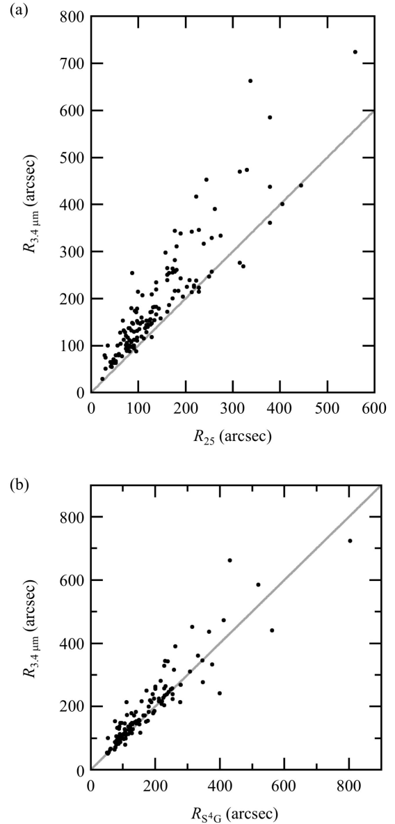
Fig. 14. Relation between the radius derived from WISE 3.4\ \mu\text{m} data in this work ( R_{3.4\ \mu\text{m}} ) and the optical radius ( R_{25} = D_{25}/2 ). The solid line indicates R_{3.4\ \mu\text{m}} = R_{25} . (b) Same as (a), but comparing with the semi-major axis in \text{S}^4\text{G} (Sheth et al. 2010).
