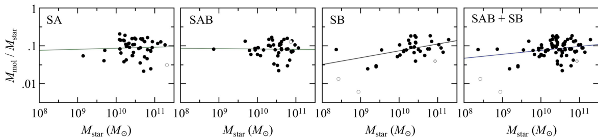
Fig. 24. Same as figure 23, but as a function of the existence of a bar or not. The galaxies not classified into these categories are not shown.
