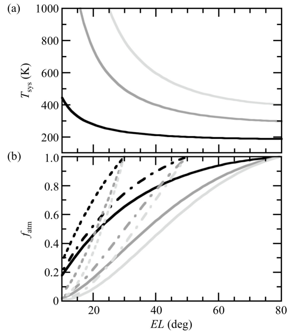
Fig. 6. (a) System noise temperature ( T_{\text{sys}} ) as a function of the elevation ( EL ). Lines for T_{\text{sys}} = 200 K (black), 350 K (dark gray), and 500 K (light gray) at EL = 50^\circ are plotted. (b) Atmospheric factor ( f_{\text{atm}} ) as a function of the elevation. The colors are the same as (a). The lines for the elevation at the culmination of 80^\circ (solid line), 50^\circ (dash-dotted line), and 30^\circ (dotted line) are plotted.
