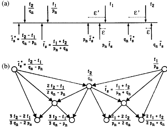
FIG. 1. (a) Schematic diagram of the frequency line, showing the relative position of \tilde{f}_s and \tilde{f}_s^* and their respective p_n, q_n harmonics that approximate f_1 and f_2 at equal distance. (b) Generalized Farey tree starting from the adjacent f_1/p_n and \tilde{f}_s^* . The first median is f_2/q_n ; at the second level we obtain \tilde{f}_s and (2f_2 - f_1)/(2q_n - p_n) , and so on.
