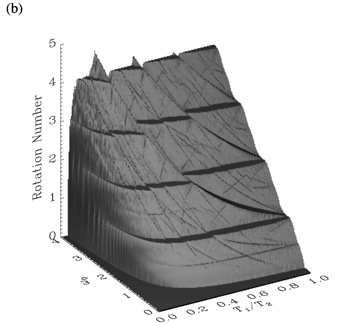
FIG. 4. Quasiperiodically forced circle map: (a) Three-frequency devil's staircase for forcing frequencies f_1 = 1, f_2 = 12/7 . (b) Devil's ramps: the rotation number as a function of the external frequency ratio and the intrinsic frequency shows the global organization of three-frequency resonances.
