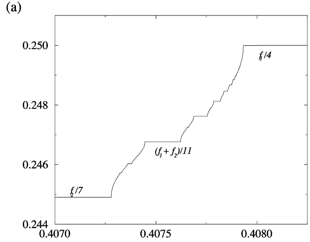
FIG. 3. The three-frequency devil's staircase for the system of ordinary differential equations of Eq. (15). The system parameters are equivalent to those of Fig. 2(b).
