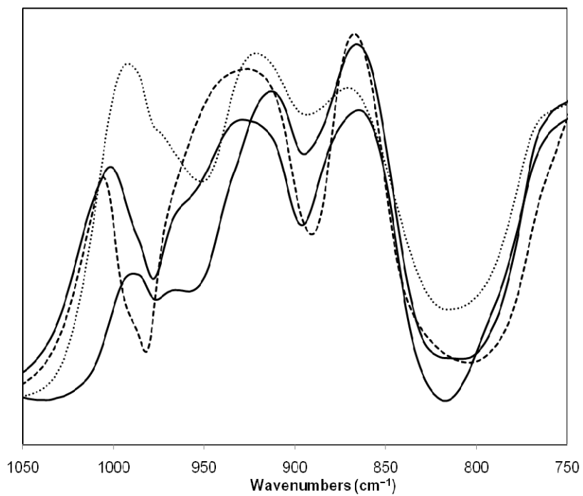
Figure 6. IR spectra of PW-S R (dashed line), PWn-S R (dotted line) and two different samples of Aza t Bu-Cu-PWn-S R (solid lines).
