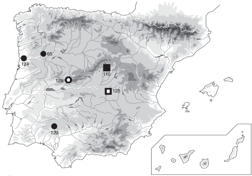
Fig. 4.— Distribution of the species of the genus Hexabathynella of the Iberian Peninsula. Each number corresponds to a sampling site (see Appendix).
