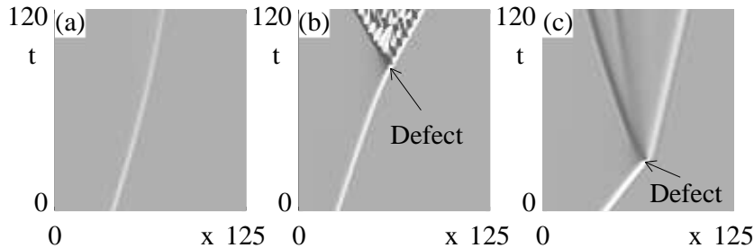
Figure 10. Evolution of perturbations of the upper branch MAWs. The coefficients c_1 and c_3 are chosen such that no saddle-node bifurcation occurs for any value of P . (a) A slowing down and spreading of the phase gradient characterizes the decay to a lower branch MAW for c_1 = 0.55 and c_3 = 2 . (b) For the same coefficients, another perturbation leads to an increase in velocity and divergence of the phase gradient. A defect occurs, from which hole-defect dynamics spreads for these coefficients. (c) For c_1 = 3 and c_3 = 0.6 a perturbed upper branch MAW leads to a defect, but defects do not percolate through the system.
