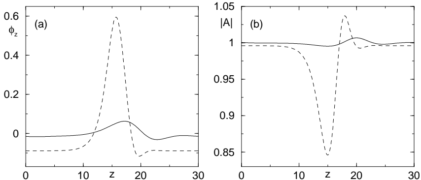
Figure 5. (a) Phase gradient and (b) amplitude profiles of a lower branch (full curve) and upper branch (dashed curve) MAW, obtained for c_1=0.6, c_3=2, P=30 .
