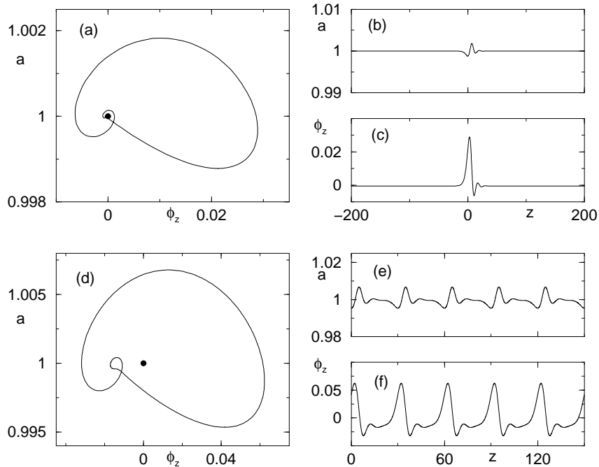
Figure 3. Examples of ODE solutions and corresponding amplitude and phase gradient profiles of MAWs. (a) Homoclinic orbit for c_1 = 0.55 and c_3 = 2 ; (b,c) corresponding profiles. (d) Limit cycle for c_1 = 0.60 , c_3 = 2 and P = 30 ; (e,f) corresponding profiles. Dots in (a,d) denote the unstable fixed point (1, 0, 0) from which these orbits emerged.
