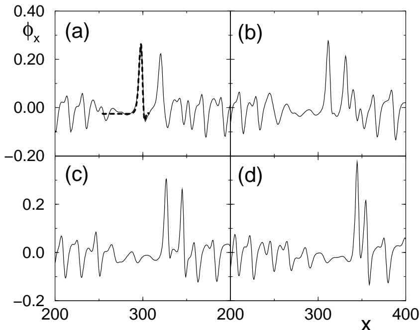
Figure 13. Local phase gradient of the chaotic field just before defect formation for c_1 = 0.65 and c_3 = 2 . Panel (a) is a snapshot of the field at a time t = 120 before the occurrence of the defect, (b), (c) and (d) are successive snapshots taken at time intervals \delta t = 30 . In (a) also the shape of the MAW at the saddle-node is superimposed (thick dashed line) on the profile.
