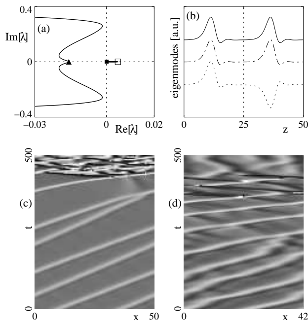
Figure 17. Results of the linear stability analysis : (a) leading part of the eigenvalue spectrum (continuous spectrum denoted by the full curve, Goldstone modes by a filled square, saddle-node by filled triangle and interaction by open square at \lambda_{int} = +0.0048 , respectively), (b) Goldstone mode (dot-dashed) and interaction eigenmode (dotted curve) for the phase compared with spatial MAW profile of the phase gradient (full curve) in L = 2P . (c,d) Space time plots showing the attraction of two periods of the same MAW initially perturbed by the interaction eigenmode. Parameters are c_1 = 0.7, c_3 = 2, P = 25 near L_3 for (a-c) and c_1 = 3, c_3 = 0.85, P = 21 near L_1 for (d).
