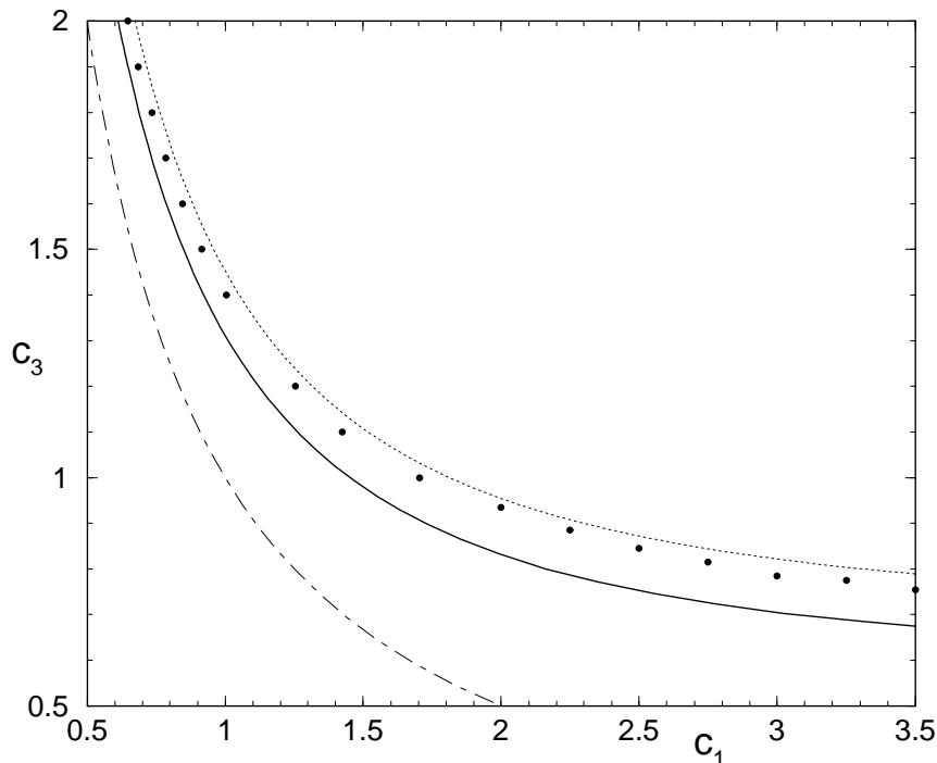
Figure 18. Space of (c_1, c_3) -coefficients for the CGLE with the Benjamin-Feir-Newell curve (dot-dashed), the lower bound P_{SN} \rightarrow \infty (full) and the stability-based estimate (dotted) for the transition from phase to defect chaos. The symbols refer to our numerical data for the appearance of defects.
