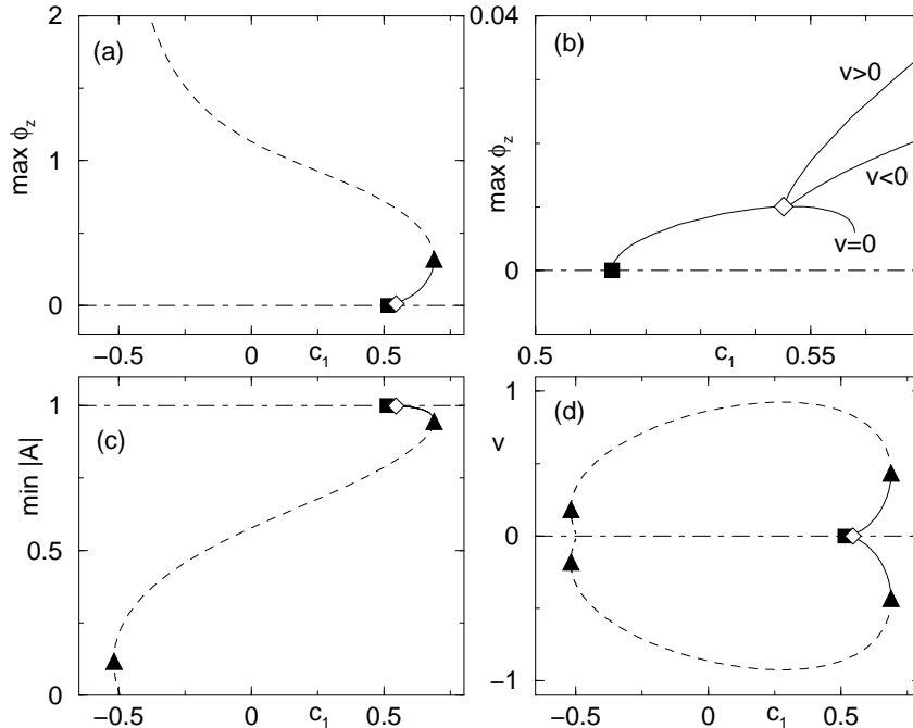
Figure 4. Bifurcation diagrams for fixed c_3 = 2 and P = 30 , showing Hopf (filled square), drift pitchfork (open diamond) and saddle-node (triangle) bifurcations. The dot-dashed line represents the homogeneously oscillating solution of the CGLE, while lower and upper branch MAWs are represented by full and dashed curves respectively. (a) Overview of the maximum phase gradient of the MAWs as function of c_1 , (b) close-up, (c) the minimum of |A| , and (d) the velocity v . For details see text.
