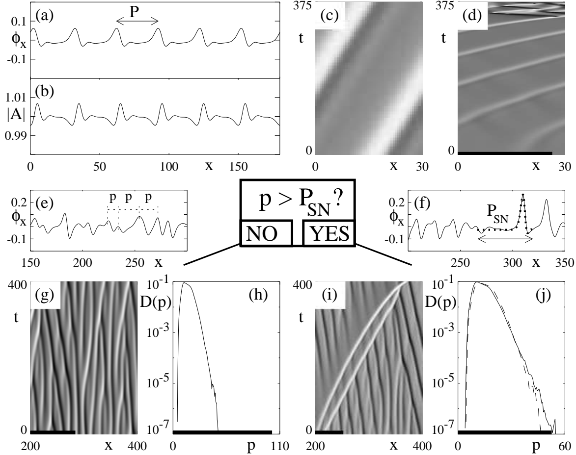
Figure 1. Summary of our main results which constitute a picture for the formation of defects from phase chaotic states. (a,b) Example of a coherent structure: phase gradient and modulus of a period P=30 MAW at c_1=0.6, c_3=2 . (c) Space time plot showing the stable propagation of the MAW from (a,b) in a small system of size P with periodic boundary conditions. Subsequent space time plots also show the phase gradient encoded in gray-scale (minima appear dark, maxima bright). (d) The same MAW as initial condition creates defects at c_1 = 0.7, c_3 = 2 where P > P_{SN} = 26.8 . Black bars above the x-axis denote the size of P_{SN} specific to the parameters of the panel. (e,g,h) Large scale chaos at c_1 = 0.63, c_3 = 2, L = 512 . (e) Snapshot of the phase gradient profile with individual inter-peak spacings p . (g) Space time evolution of phase chaos and (h) distribution D(p) showing p \ll P_{SN} and no defects. A transient of t \approx 10^4 is not shown. (f,i,j) Large scale chaos at c_1 = 0.65, c_3 = 2, L = 512 . (f) Snapshot of the phase gradient profile t = 120 before the first defect forms and the MAW (dotted, P = P_{SN} ) overlaid onto the long structure. (i) Transient phase chaos with a fast and long structure traveling through the system which eventually nucleates defect chaos at t = 400, x = 360 (a transient of t \approx 10^4 is not shown). A snapshot of this structure was shown in (f). (j) The tail of the distribution of p reaches p > P_{SN} due to the long structure; this leads to the break down of phase chaos. The distribution D(p) shown in (h) is also reported (dashed line). From the comparison of the two it is evident that the distributions do not modify dramatically when c_1 is increased, while P_{SN} decreases noticeably.
