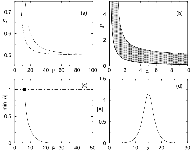
Figure 6. (a) Location of Hopf (dashed curve) and drift pitchfork bifurcation (dotted curve) in c_1, P space for c_3 = 2.0 . (b) The shaded area reported in the c_1, c_3 coefficient space indicates where the drift pitchfork bifurcation does occur. The thick full curve in (a,b) indicates the Benjamin-Feir-Newell instability for infinite domains. (c) Example of a bifurcation diagram for large values of the coefficients c_1 = 10, c_3 = 5 where the drift pitchfork bifurcation does not occur. For increasing P the MAW solutions approach regular arrays of stationary pulses; an example of such a pulse is shown in (d) for P = 30 .
