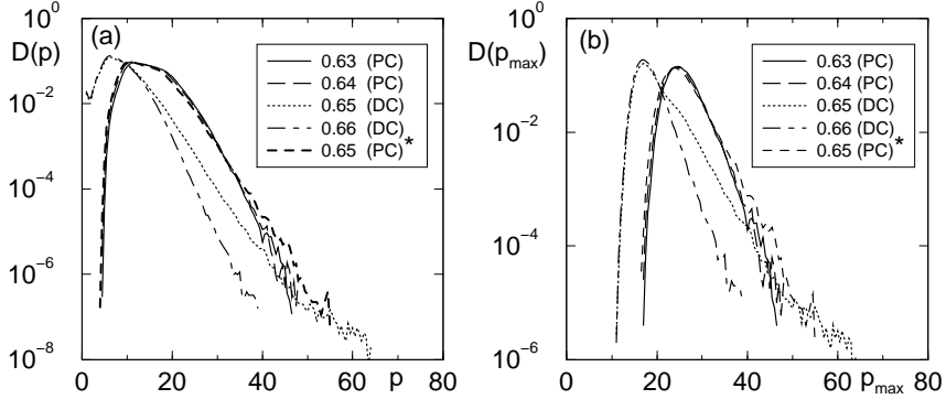
Figure 15. Probability densities (a) D(p) and (b) D(p_{max}) for c_3 = 2 and various values of c_1 reported in a lin-log scale. The data are for a system size L = 512 and for integration times ranging from t = 5 \times 10^5 for c_1 = 0.63, 0.64, 0.66 and 0.65 (PC)* to t = 2.5 \times 10^6 for c_1 = 0.65 (DC). The labels DC and PC indicate that we are in presence or absence of defects, respectively. The label (PC)* refers to the regime before defect formation at c_1 = 0.65 .
