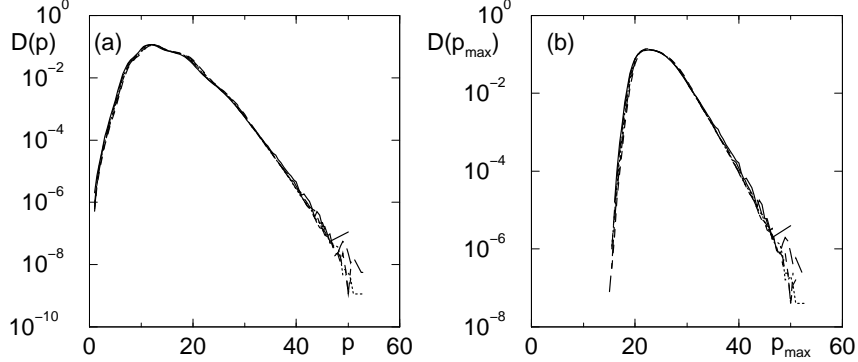
Figure 14. Probability densities (a) D(p) and (b) D(p_{max}) for c_1 = 3 and various values of c_3 on a lin-log scale. The curves refer to c_3 below c_3^* = 0.79 (namely to c_3 = 0.77 and 0.78 ), as well as to values corresponding to the defect chaotic regime: c_3 = 0.79, 0.80 and 0.81 . The system size was L = 512 and the integration times where t = 5 \times 10^5 for c_3 = 0.81 , t = 5 \times 10^6 for c_3 = 0.80 and t = 25 \times 10^6 for all other values.
