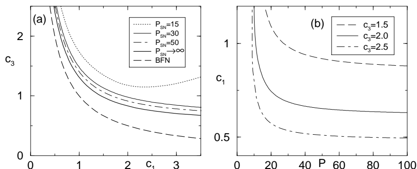
Figure 7. Locations of the saddle-node bifurcations in the c_1, c_3 plane (a) and the P, c_1 plane (b). BFN denotes the Benjamin-Feir-Newell curve.
