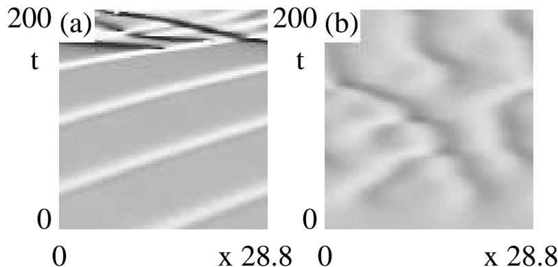
Figure 12. Defect formation at c_3 = 2, c_1 = 0.7 . (a) Defect formation. As initial condition we took a lower branch MAW with P < P_{SN} = 26.8 which we embedded in a background of zero wavenumber. The system size L here is equal to 28.8, which is larger than P_{SN} and a defect is formed; for L < P_{SN} this defect formation does not take place. (b) Random initial conditions in general evolve to MAW like structures with P < P_{SN} which do not lead to defects; the “critical” nucleus that leads to defect formation has a rather small basin of attraction here.
