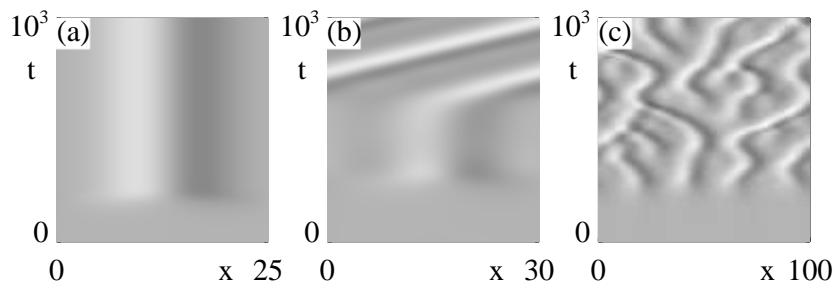
Figure 9. The evolution of an unstable homogeneous state towards lower branch MAW dynamics, for c_1 = 3 and c_3 = 0.6 . The coefficients c_1 and c_3 are chosen such that no saddle-node bifurcation occurs for any P . (a) Evolution towards a stable stationary lower branch MAW for system size L = 25 and (b) towards a stable drifting lower branch MAW for system size L = 30 . Note that for the coefficients chosen, the drift pitchfork bifurcation occurs at P = 27.7 . (c) Evolution towards phase chaos for system size L = 100 . Incoherent evolution of structures characterized by local concentrations of phase gradients can be clearly observed. We think of these structures as “near” MAWs.
