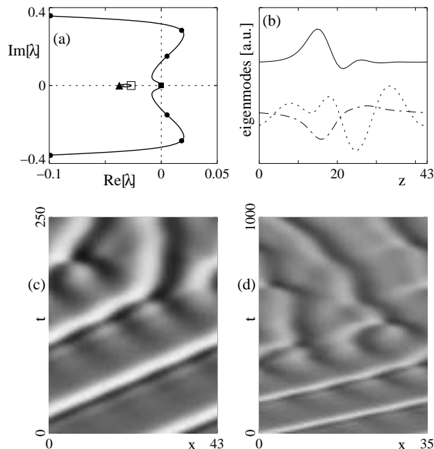
Figure 16. Results of the linear stability analysis : (a) leading part of the eigenvalue spectrum (continuous spectrum denoted by the full curve, Goldstone modes by a filled square, saddle-node by filled triangle, interaction by open square and splitting modes in L = P by dots, respectively), (b) splitting eigenmodes (dot-dashed and dotted, \lambda_{split} = 0.018 \pm 0.28i ) of the phase in L = P compared with spatial MAW profile of the phase gradient (full curve). (c,d) Space time plots showing the splitting of a MAW initially perturbed by small noise. Parameters are c_1 = 3, c_3 = 0.72, P = 43 near L_1 for (a-c) and c_1 = 0.65, c_3 = 2, P = 35 near L_3 for (d).
