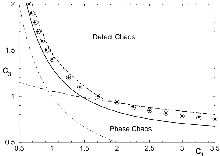
Figure 2. Phase diagram of the CGLE, showing the Benjamin-Feir-Newell curve (thin dot-dashed) where the transition from stable homogeneous oscillations to phase chaos takes place. The curves L_1 (long dashed), L_2 (thin dashed) and L_3 (dashed) as obtained in [17,19] separate the various chaotic states. The filled circles correspond to our estimates of the L_1 and L_3 transitions based on direct simulations of the CGLE along the 17 cuts in coefficient space that we studied. The open circles correspond to the location in coefficient space where the maximal inter-peak spacing p_{max} is equal to the maximal MAW period P_{SN} . Only small discrepancies between these two can be observed. Finally the full curve shows the P_{SN} \rightarrow \infty limit which we conjecture to be a lower boundary for the transition from phase to defect chaos.
