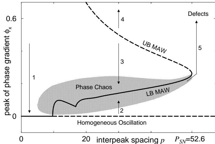
Figure 8. Illustration of the relation between MAW structures and phase chaos for c_1 = 0.65 , c_3 = 2 . Both for MAWs and for an extended profile obtained from a phase chaotic state one can extract the values of subsequent phase gradient peaks (vertical axis) and their inter-peak spacing (horizontal axis). The curves show the bifurcation diagram for the lower branch (LB) MAWs and upper branch (UB) MAWs while the shaded area indicates the typical values for near-MAW structures that occur in phase chaos. Full (dashed) curves denote stable (unstable) solutions for system size L = p . Arrows show the typical evolutions of near-MAWs. The coefficients here are equal to those in Fig. 1 (f,i,j) and for this case we have found that phase chaos is only a long lived transient: the shaded area reaches P_{SN} just before defects appear.
