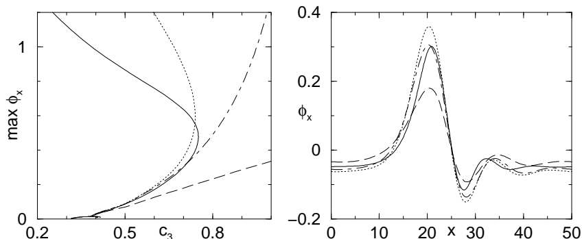
Figure 11. Comparison of different phase expansions : Eq.(4) (dotted), Eq.(4) without the last term (dot-dashed), Kuramoto-Sivashinsky Eq. (dashed) and CGLE (full curve). Parameters are c_1 = 3.5, \nu = 0, P = 50 . (a) Bifurcation diagrams and (b) spatial profiles of lower branch coherent structures at c_3 = 0.7 .
