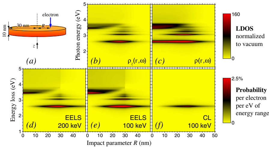
FIG. 2 (color online). Relation between EELS and LDOS in planar geometries. (a) We consider an Ag disk of height 10 nm and radius 30 nm. The electrons move along z , perpendicular to the disk. The EELS probability for 200-keV (d) and 100-keV (e) electrons mimics closely the z -projected LDOS in a plane 10 nm above the disk (b), and less closely the unprojected LDOS ( \rho = \rho_x + \rho_y + \rho_z ) (c). The CL emission only picks up part of the inelastic signal (f).
