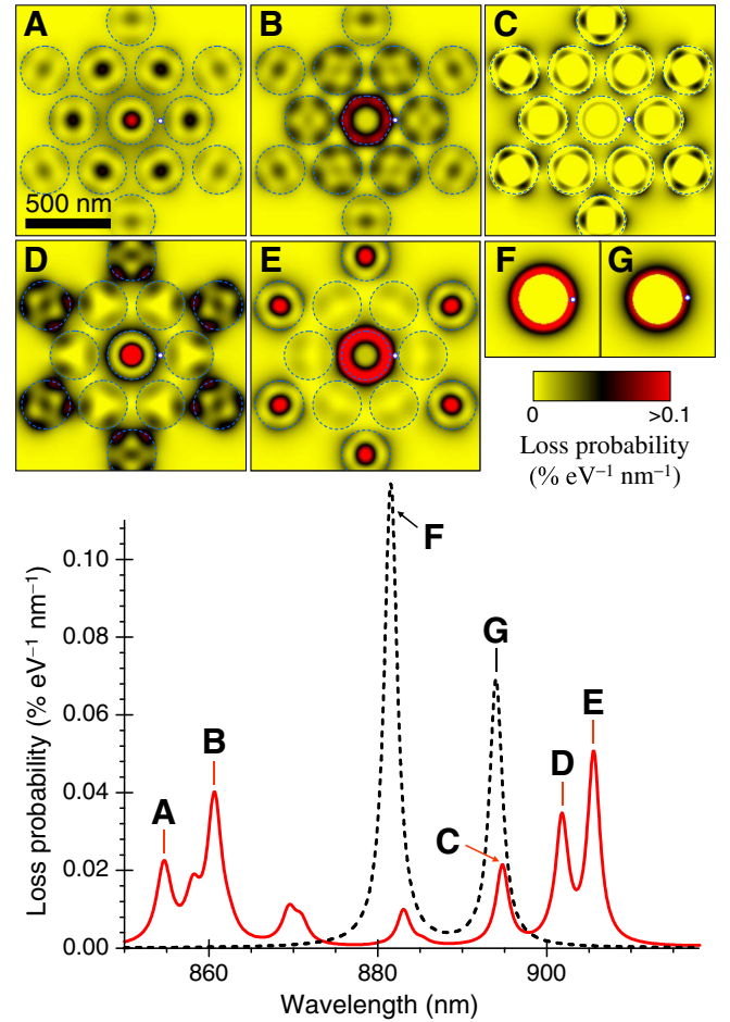
FIG. 1 (color online). EELS probability for 200-keV electrons moving parallel to an array of 13 Si nanowires of 300 nm in diameter (solid curve), as compared to an isolated nanowire (broken curve). The nanowires are arranged in a hexagonal lattice with a period of 350 nm. The contour-plot insets show the impact-parameter dependence of the EELS probability for selected energy losses (labeled A–G), with the position of the electron beam considered in the curves indicated by an open symbol and the cylinder contours shown by dashed curves.
