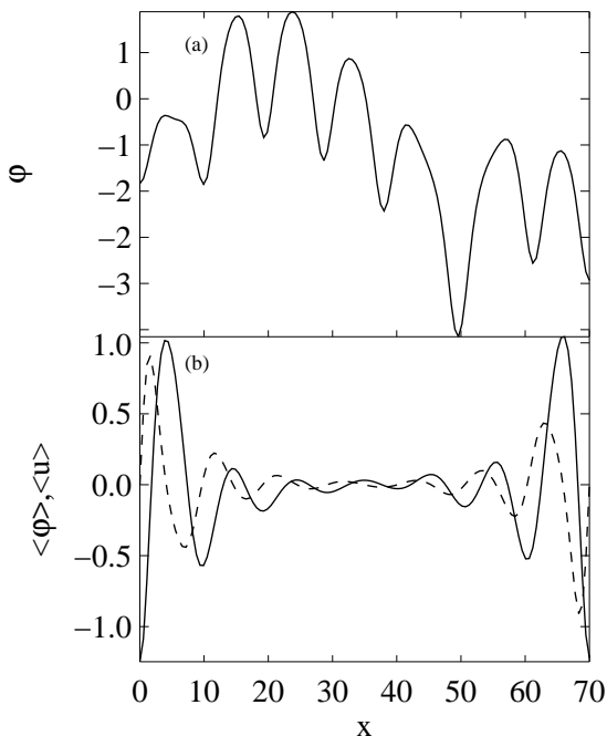
FIG. 1. Results from simulations of the one-dimensional Kuramoto-Sivashinsky equation with stress-free boundary conditions. System size L = 70 . a) A characteristic front \varphi at time t = 1000 . b) The time average of the front \varphi (continuous line) and of u (dashed).
