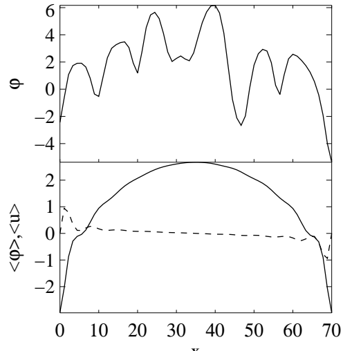
FIG. 4. a) A central horizontal x cut of the configuration shown in the left panel of Fig. 3. b) Solid: a central horizontal cut of the time average of the front \varphi for the same parameter values; dashed: the same cut for the time average of \varphi_x .
