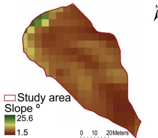
Figure 3. Slope map.
