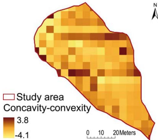
Figure 4. Concavity-convexity map.
