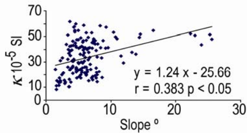
Figure 9. Linear regression between slope gradient and kis.
