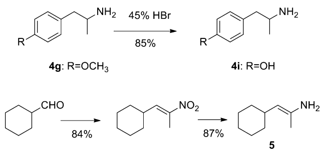
Scheme 2 Synthesis of amines 4i and 5 .
