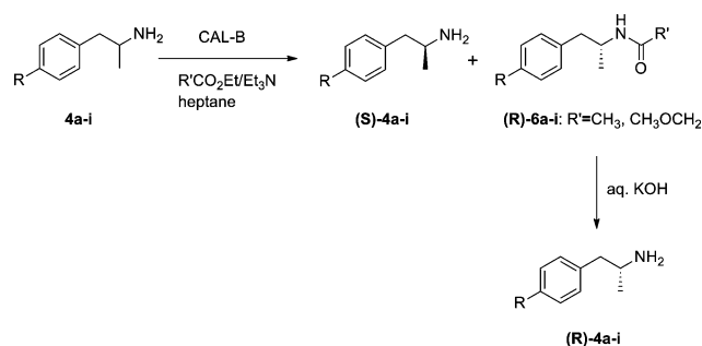
Scheme 3 Enzymatic resolution of racemic amines 4a–i .
