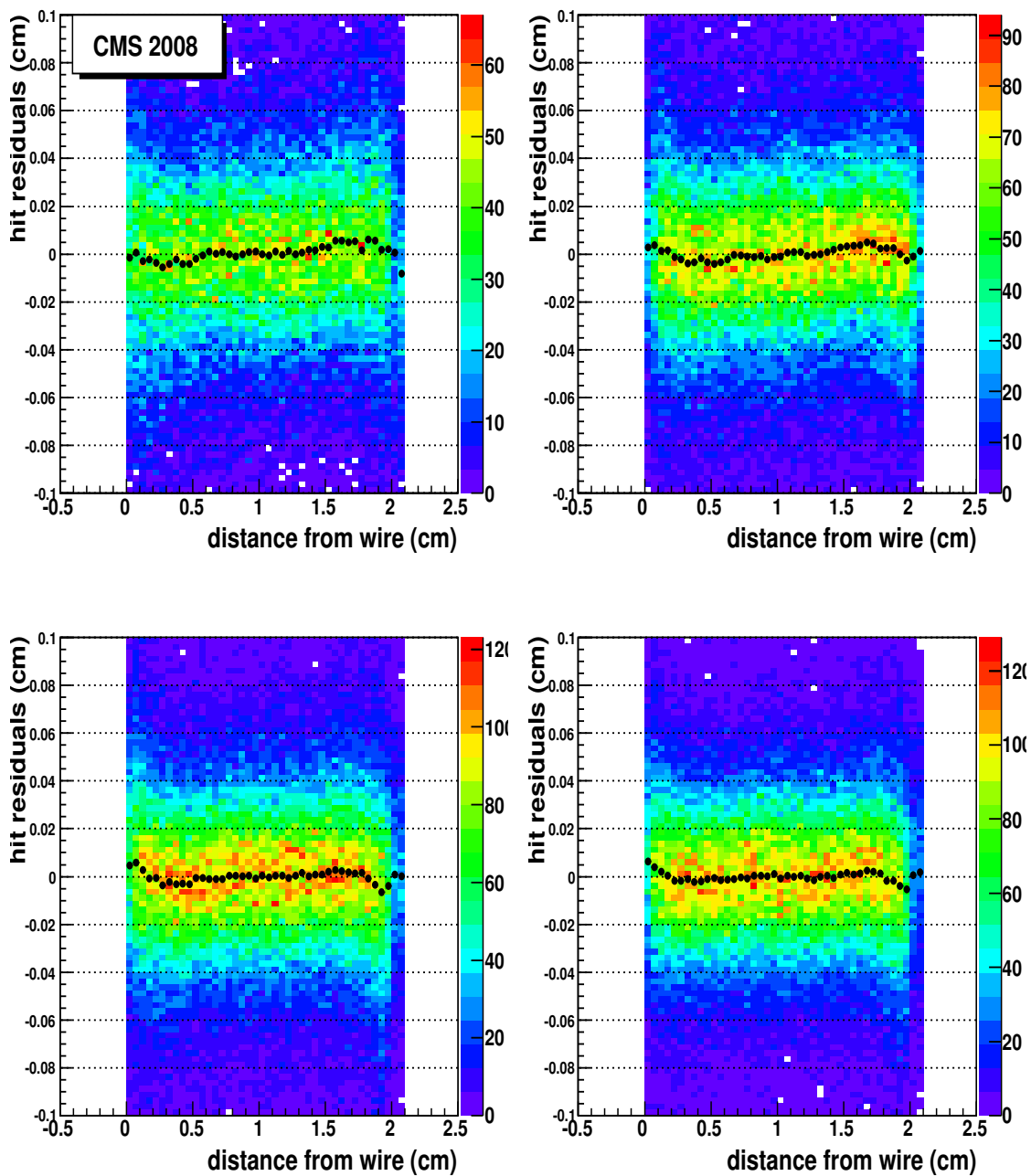
Figure 8. Plot of residuals vs hit position in a DT cell, for the chambers of YB–2, sector 4; the plot profile is shown by the points. Top plots: MB1 (left) and MB2 (right). Bottom plots: MB3 (left) and MB4 (right).
